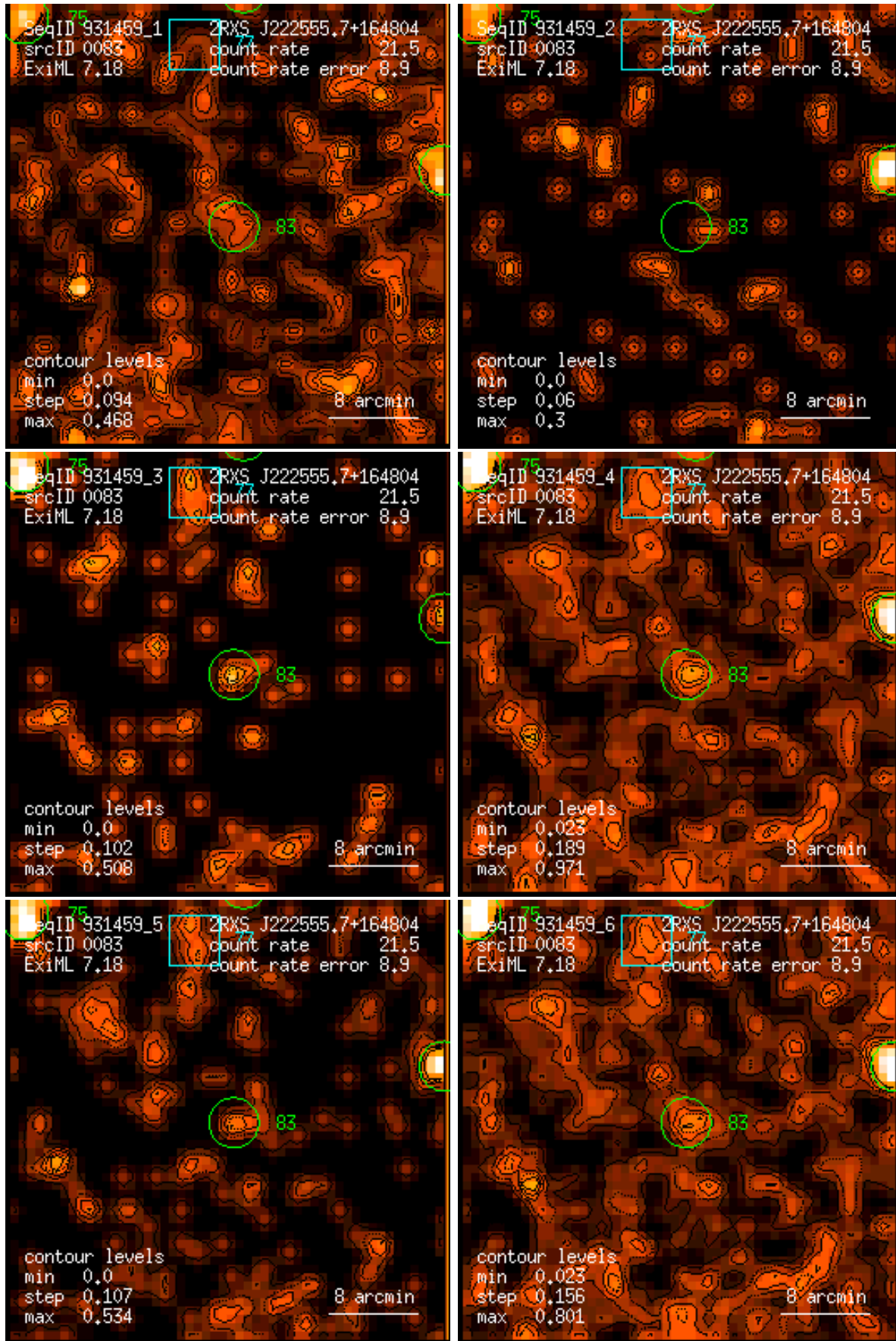
Figure 83: RASS 931459: detection 0083: band rate images, Gaussian filter: (1) PSPC channels 11 – 41, (2) 52 – 90, (3) 91 – 201, (4) 11 – 235, (5) 52 – 201, (6) 11 – 201. Broad band rates in counts/ks. Band rate contour levels in counts/ks/arcmin 2 .
