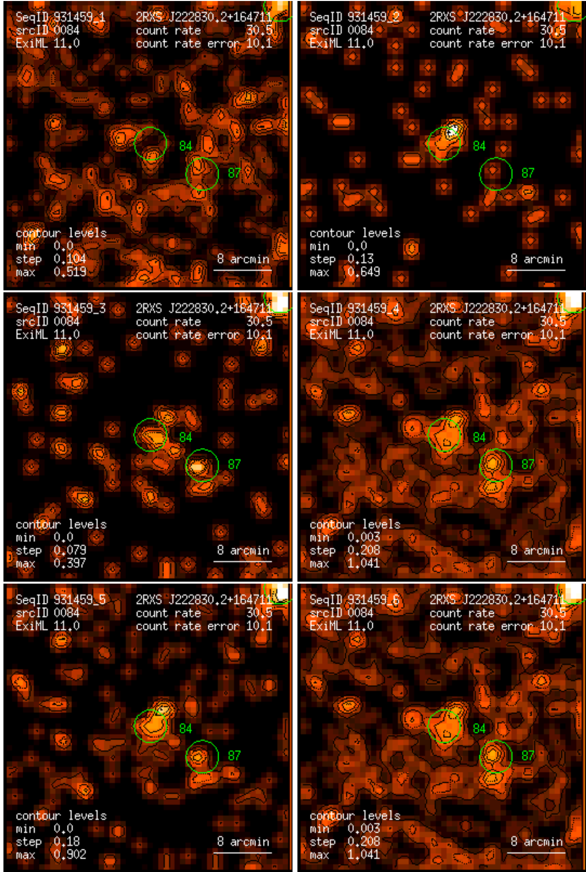
Figure 84: RASS 931459: detection 0084: band rate images, Gaussian filter: (1) PSPC channels 11 – 41, (2) 52 – 90, (3) 91 – 201, (4) 11 – 235, (5) 52 – 201, (6) 11 – 201. Broad band rates in counts/ks. Band rate contour levels in counts/ks/arcmin 2 .
