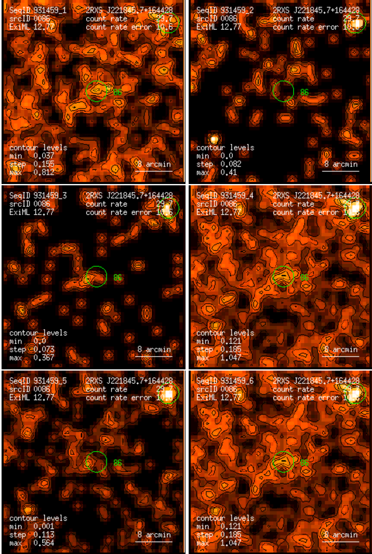
Figure 86: RASS 931459: detection 0086: band rate images, Gaussian filter: (1) PSPC channels 11 – 41, (2) 52 – 90, (3) 91 – 201, (4) 11 – 235, (5) 52 – 201, (6) 11 – 201. Broad band rates in counts/ks. Band rate contour levels in counts/ks/arcmin 2 .
