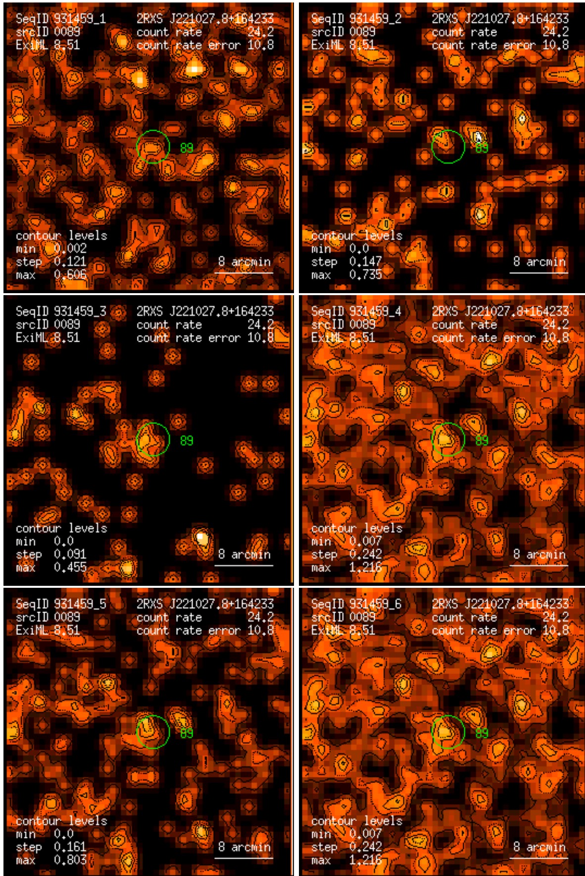
Figure 89: RASS 931459: detection 0089: band rate images, Gaussian filter: (1) PSPC channels 11 – 41, (2) 52 – 90, (3) 91 – 201, (4) 11 – 235, (5) 52 – 201, (6) 11 – 201. Broad band rates in counts/ks. Band rate contour levels in counts/ks/arcmin 2 .
