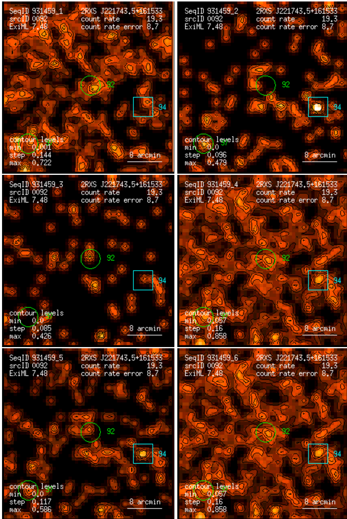
Figure 92: RASS 931459: detection 0092: band rate images, Gaussian filter: (1) PSPC channels 11 – 41, (2) 52 – 90, (3) 91 – 201, (4) 11 – 235, (5) 52 – 201, (6) 11 – 201. Broad band rates in counts/ks. Band rate contour levels in counts/ks/arcmin 2 .
