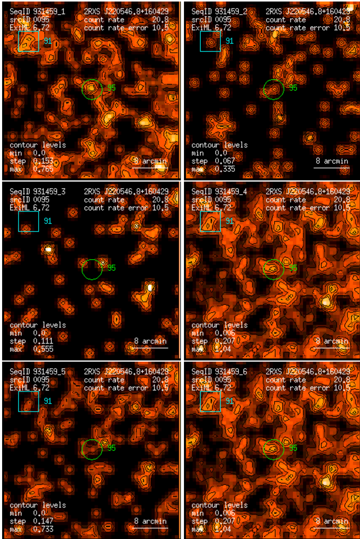
Figure 95: RASS 931459: detection 0095: band rate images, Gaussian filter: (1) PSPC channels 11 – 41, (2) 52 – 90, (3) 91 – 201, (4) 11 – 235, (5) 52 – 201, (6) 11 – 201. Broad band rates in counts/ks. Band rate contour levels in counts/ks/arcmin 2 .
