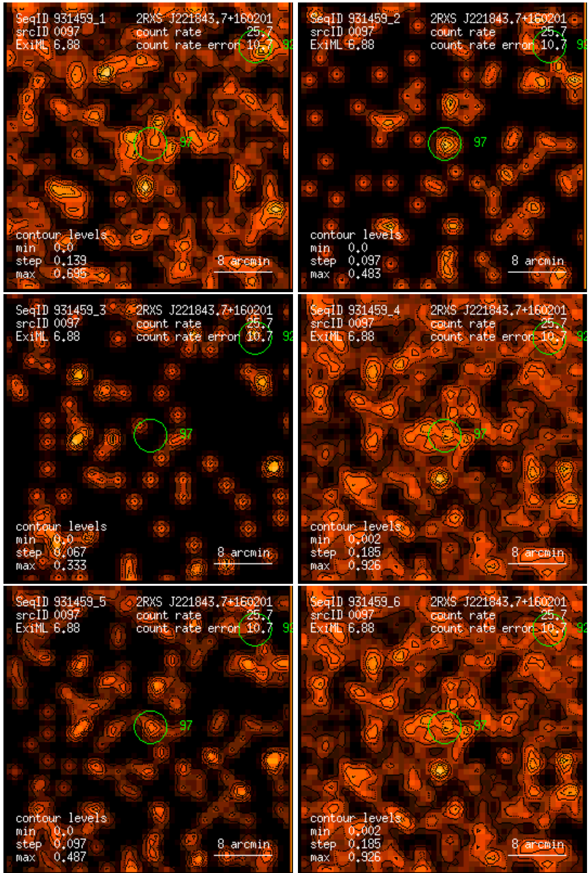
Figure 97: RASS 931459: detection 0097: band rate images, Gaussian filter: (1) PSPC channels 11 – 41, (2) 52 – 90, (3) 91 – 201, (4) 11 – 235, (5) 52 – 201, (6) 11 – 201. Broad band rates in counts/ks. Band rate contour levels in counts/ks/arcmin 2 .
