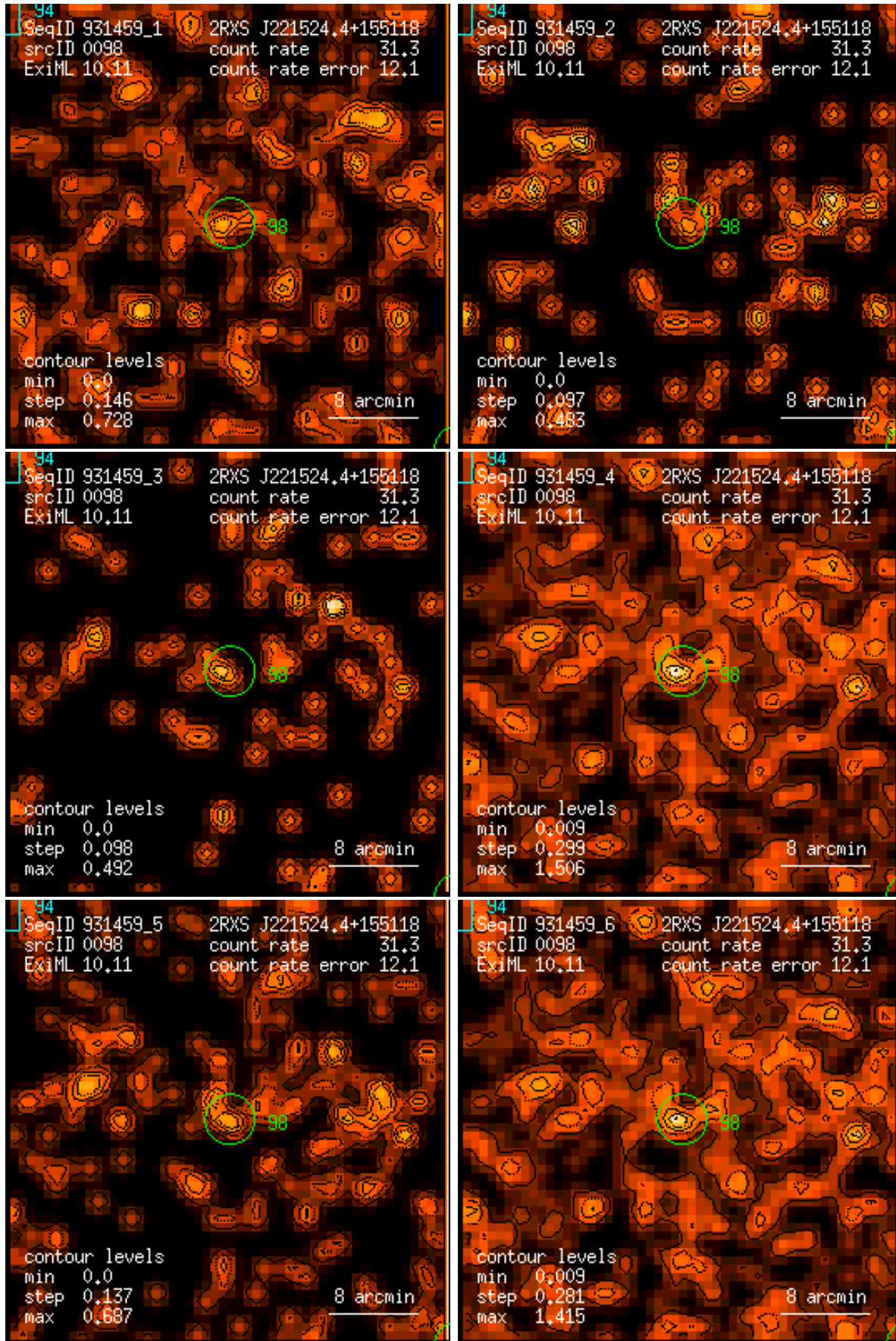
Figure 98: RASS 931459: detection 0098: band rate images, Gaussian filter: (1) PSPC channels 11 – 41, (2) 52 – 90, (3) 91 – 201, (4) 11 – 235, (5) 52 – 201, (6) 11 – 201. Broad band rates in counts/ks. Band rate contour levels in counts/ks/arcmin 2 .
