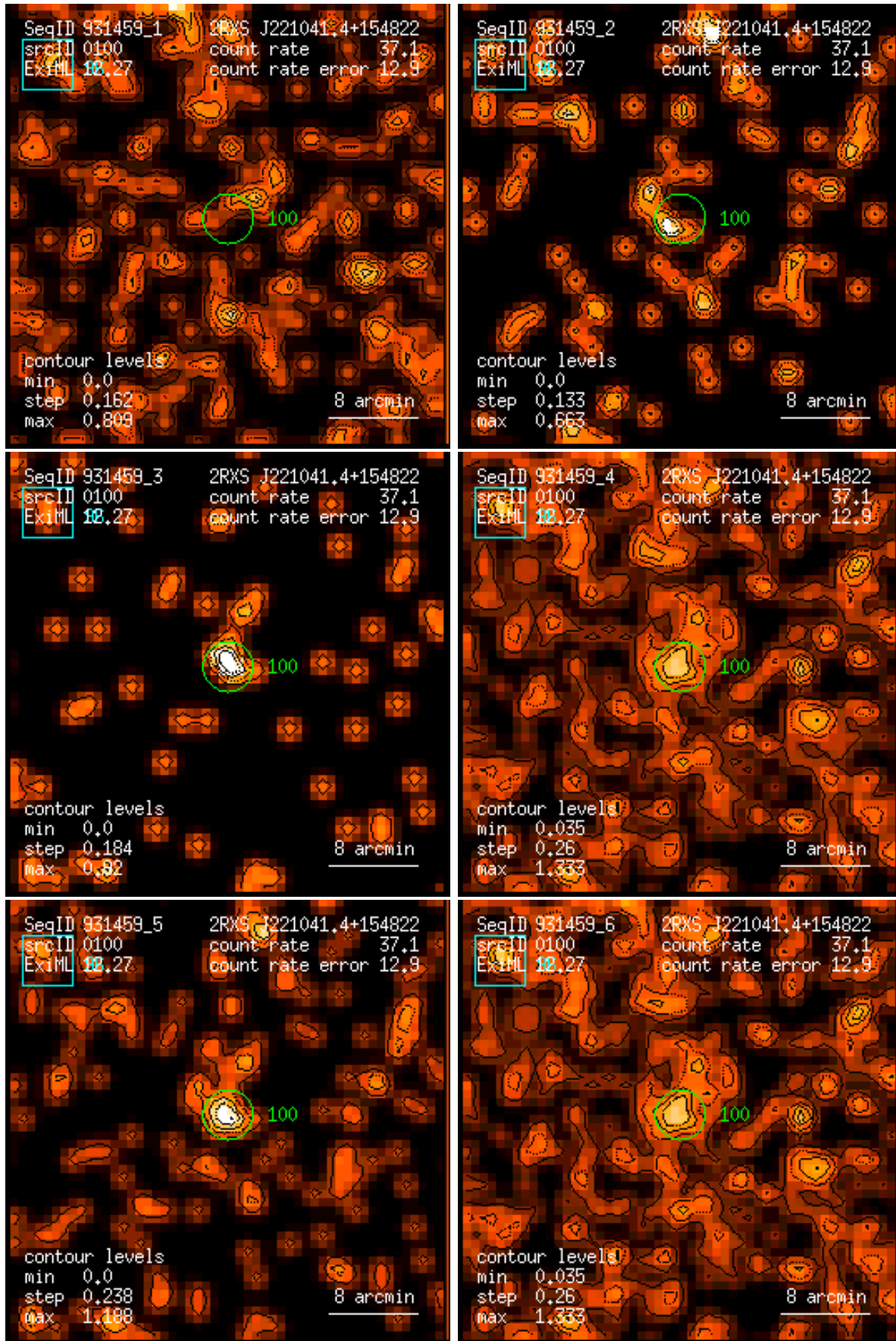
Figure 100: RASS 931459: detection 0100: band rate images, Gaussian filter: (1) PSPC channels 11 – 41, (2) 52 – 90, (3) 91 – 201, (4) 11 – 235, (5) 52 – 201, (6) 11 – 201. Broad band rates in counts/ks. Band rate contour levels in counts/ks/arcmin 2 .
