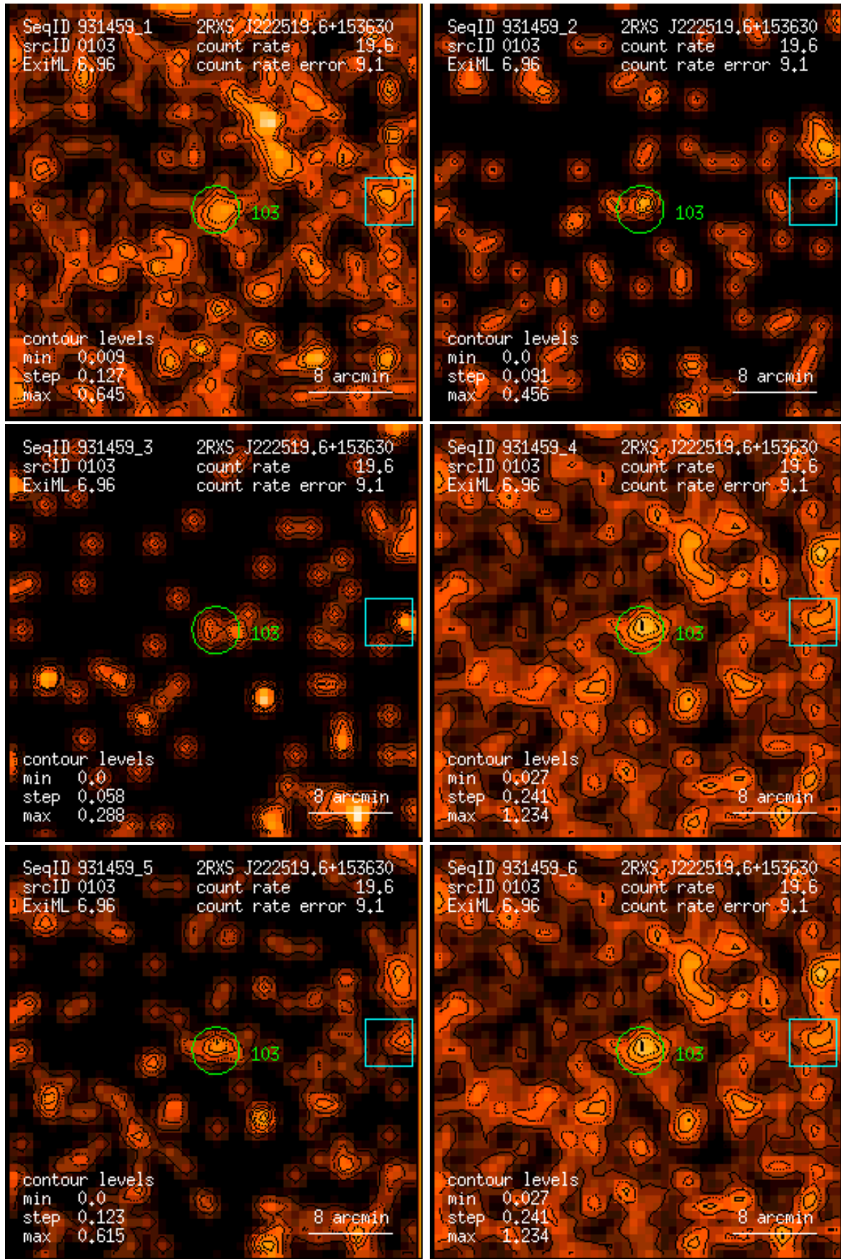
Figure 103: RASS 931459: detection 0103: band rate images, Gaussian filter: (1) PSPC channels 11 – 41, (2) 52 – 90, (3) 91 – 201, (4) 11 – 235, (5) 52 – 201, (6) 11 – 201. Broad band rates in counts/ks. Band rate contour levels in counts/ks/arcmin 2 .
