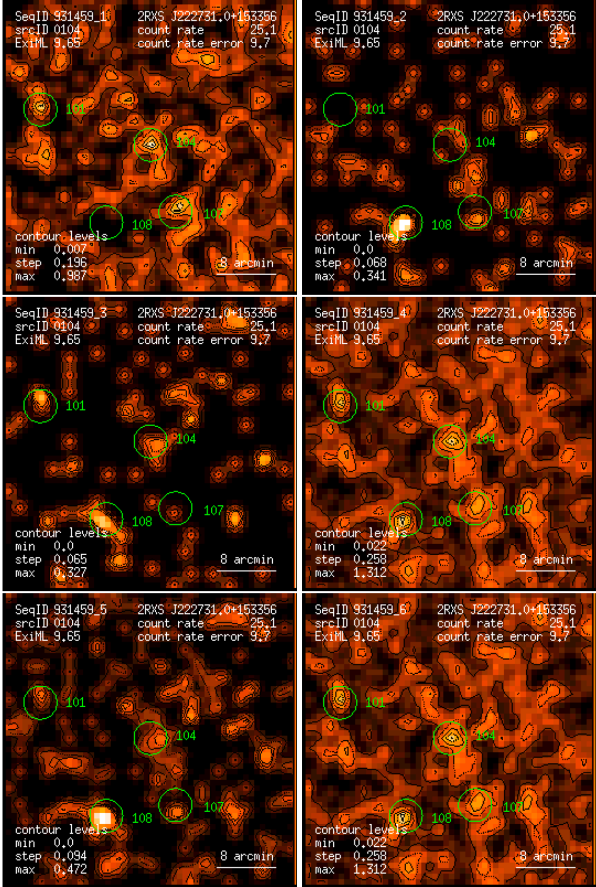
Figure 104: RASS 931459: detection 0104: band rate images, Gaussian filter: (1) PSPC channels 11 – 41, (2) 52 – 90, (3) 91 – 201, (4) 11 – 235, (5) 52 – 201, (6) 11 – 201. Broad band rates in counts/ks. Band rate contour levels in counts/ks/arcmin 2 .
