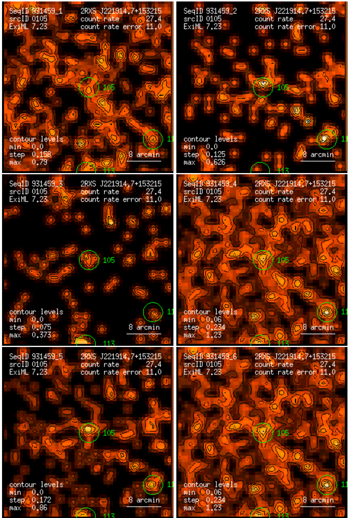
Figure 105: RASS 931459: detection 0105: band rate images, Gaussian filter: (1) PSPPC channels 11 – 41, (2) 52 – 90, (3) 91 – 201, (4) 11 – 235, (5) 52 – 201, (6) 11 – 201. Broad band rates in counts/ks. Band rate contour levels in counts/ks/arcmin 2 .
