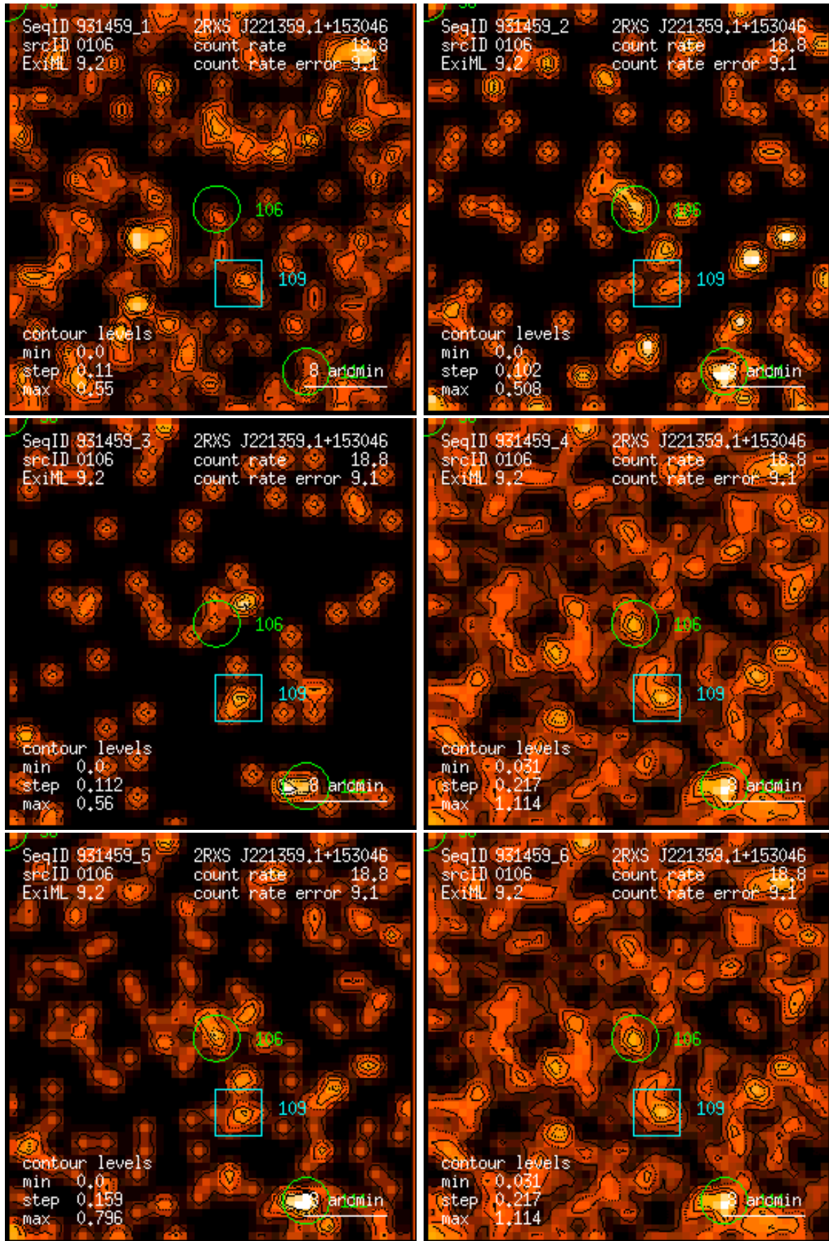
Figure 106: RASS 931459: detection 0106: band rate images, Gaussian filter: (1) PSPC channels 11 – 41, (2) 52 – 90, (3) 91 – 201, (4) 11 – 235, (5) 52 – 201, (6) 11 – 201. Broad band rates in counts/ks. Band rate contour levels in counts/ks/arcmin 2 .
