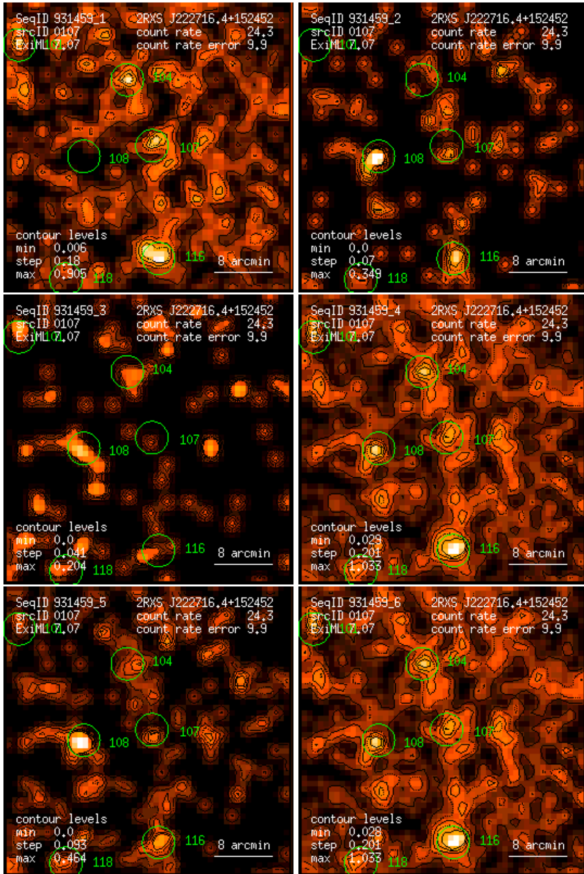
Figure 107: RASS 931459: detection 0107: band rate images, Gaussian filter: (1) PSPC channels 11 – 41, (2) 52 – 90, (3) 91 – 201, (4) 11 – 235, (5) 52 – 201, (6) 11 – 201. Broad band rates in counts/ks. Band rate contour levels in counts/ks/arcmin 2 .
