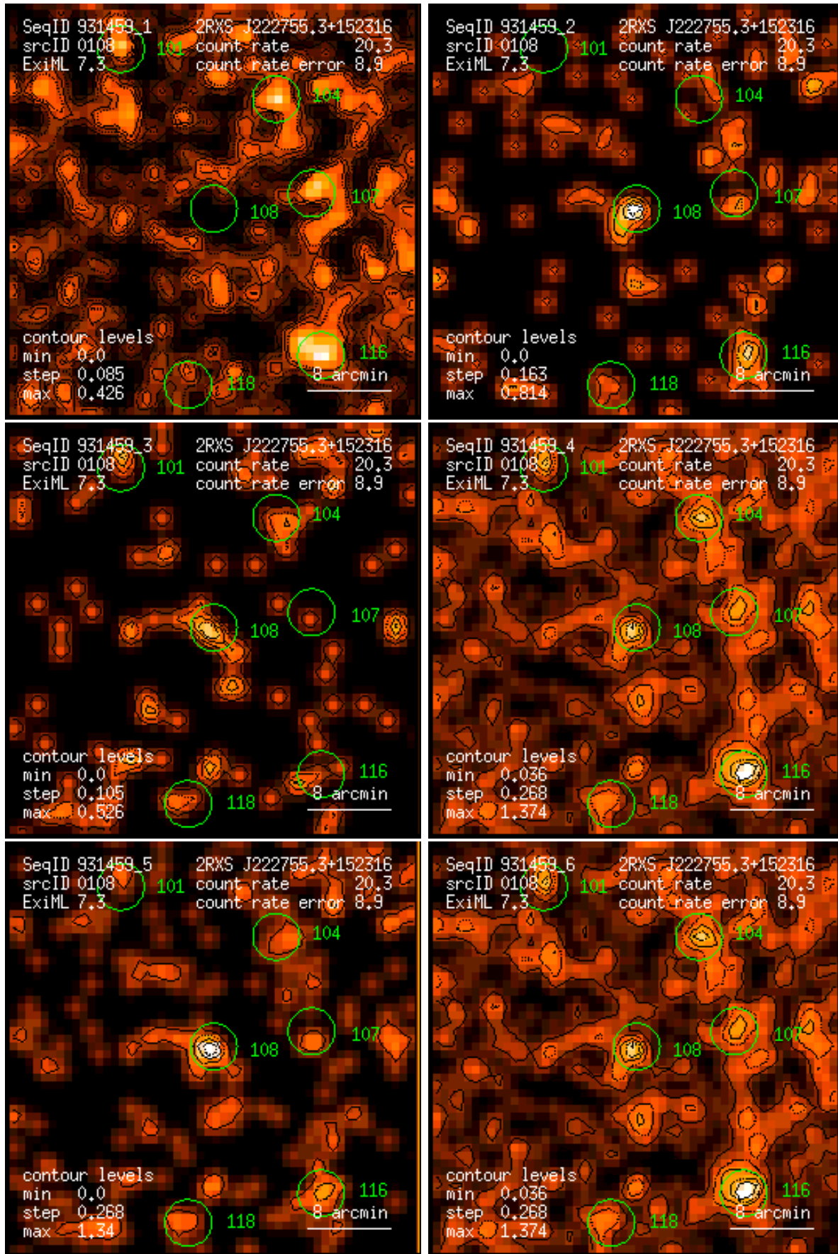
Figure 108: RASS 931459: detection 0108: band rate images, Gaussian filter: (1) PSPC channels 11 – 41, (2) 52 – 90, (3) 91 – 201, (4) 11 – 235, (5) 52 – 201, (6) 11 – 201. Broad band rates in counts/ks. Band rate contour levels in counts/ks/arcmin 2 .
