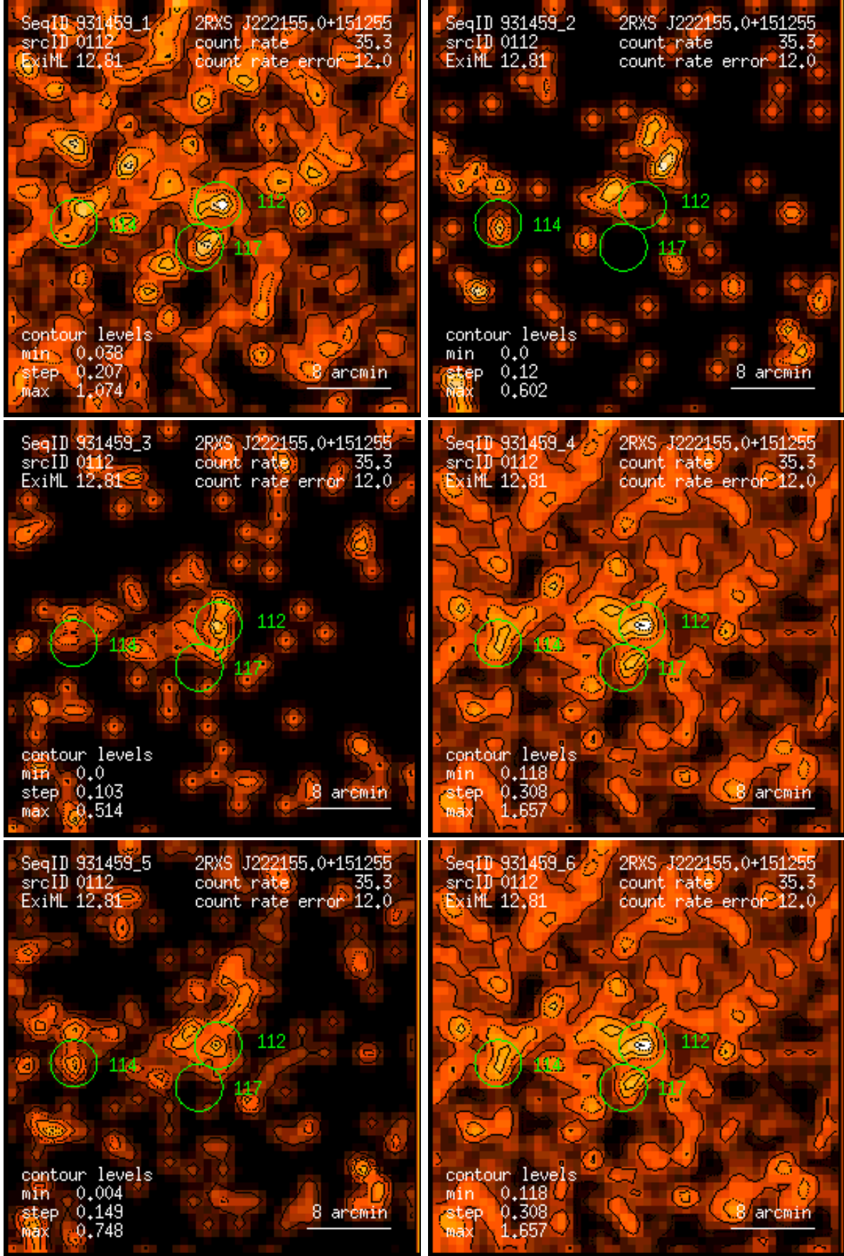
Figure 112: RASS 931459: detection 0112: band rate images, Gaussian filter: (1) PSPC channels 11 – 41, (2) 52 – 90, (3) 91 – 201, (4) 11 – 235, (5) 52 – 201, (6) 11 – 201. Broad band rates in counts/ks. Band rate contour levels in counts/ks/arcmin 2 .
