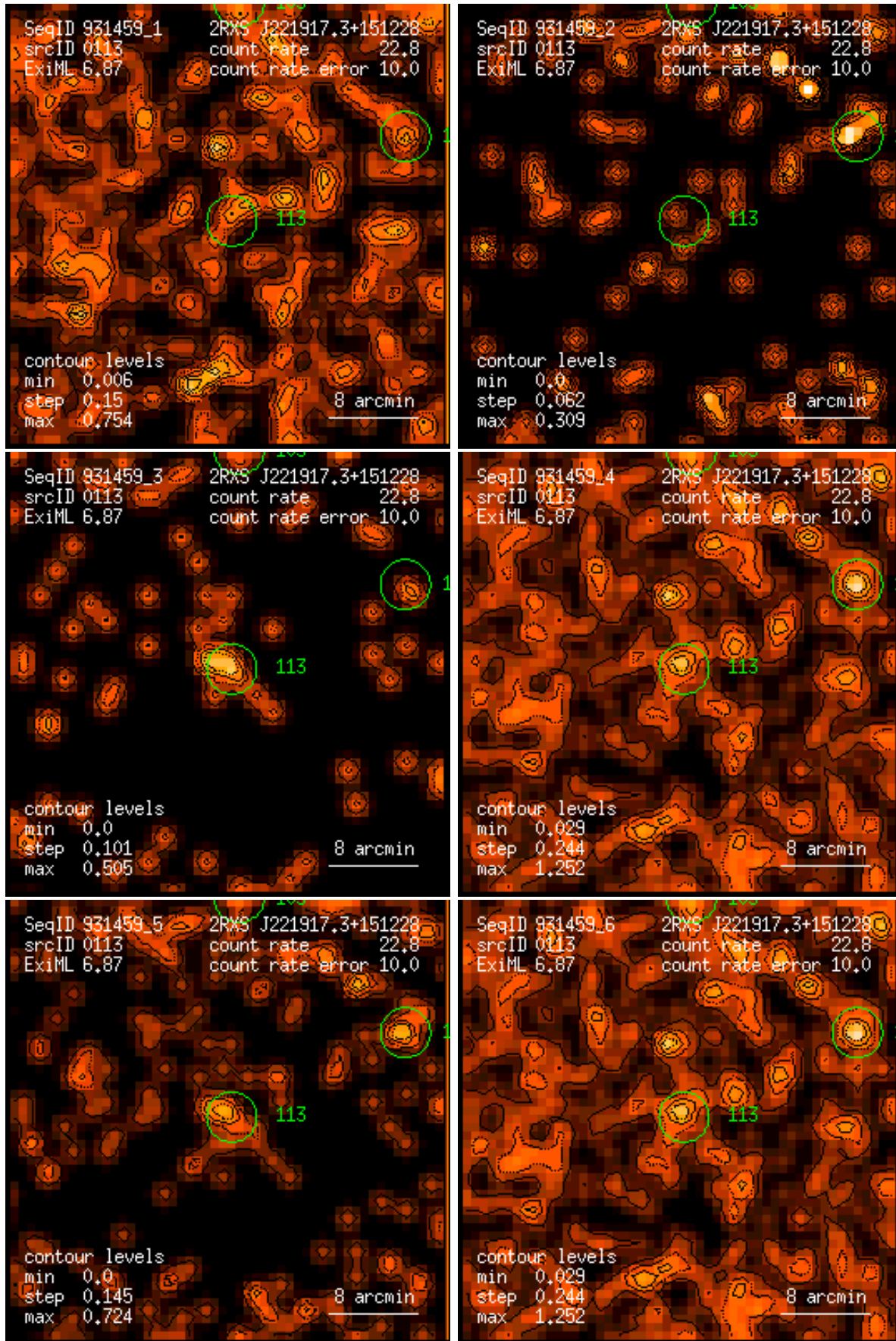
Figure 113: RASS 931459: detection 0113: band rate images, Gaussian filter: (1) PSPC channels 11 – 41, (2) 52 – 90, (3) 91 – 201, (4) 11 – 235, (5) 52 – 201, (6) 11 – 201. Broad band rates in counts/ks. Band rate contour levels in counts/ks/arcmin 2 .
