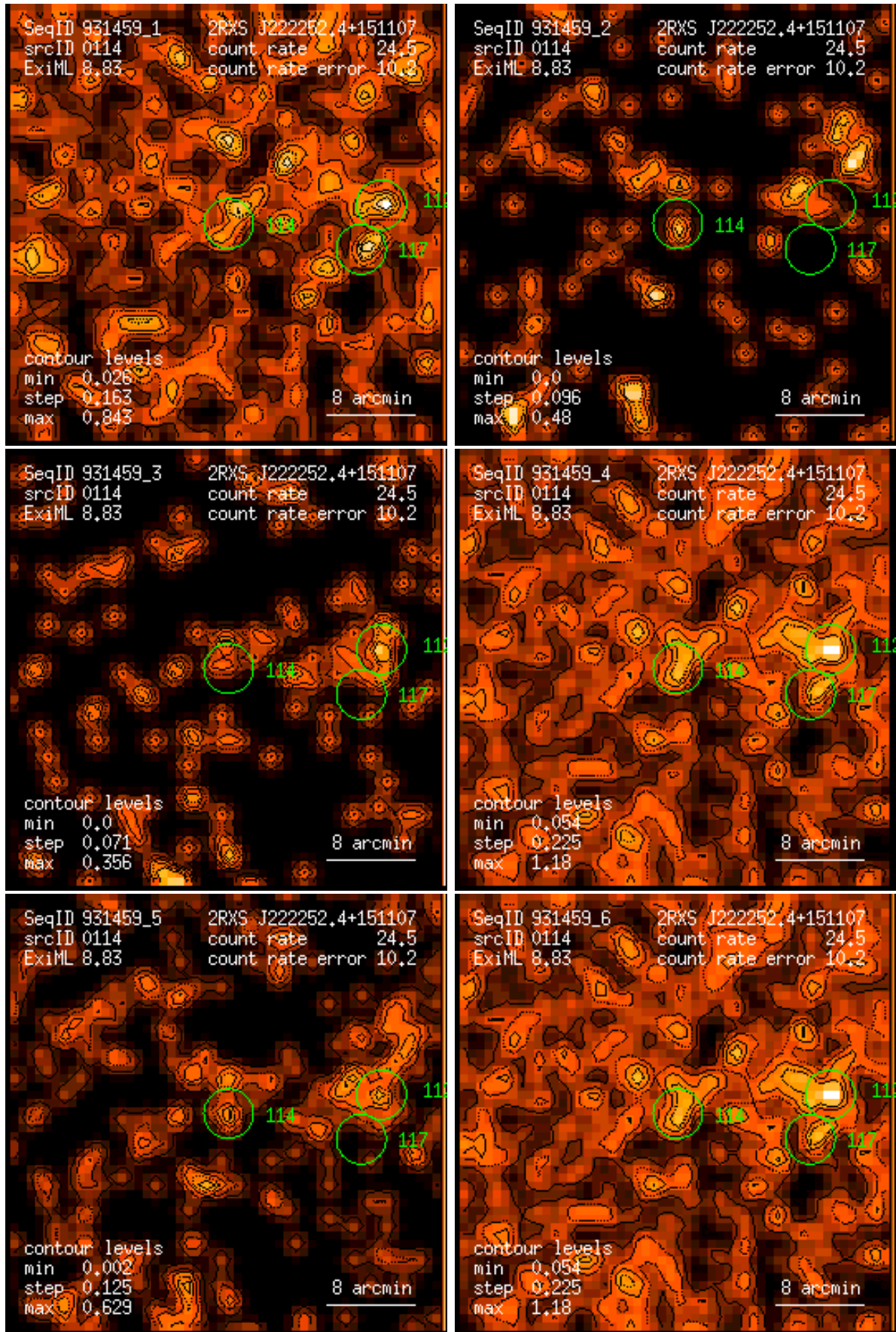
Figure 114: RASS 931459: detection 0114: band rate images, Gaussian filter: (1) PSPC channels 11 – 41, (2) 52 – 90, (3) 91 – 201, (4) 11 – 235, (5) 52 – 201, (6) 11 – 201. Broad band rates in counts/ks. Band rate contour levels in counts/ks/arcmin 2 .
