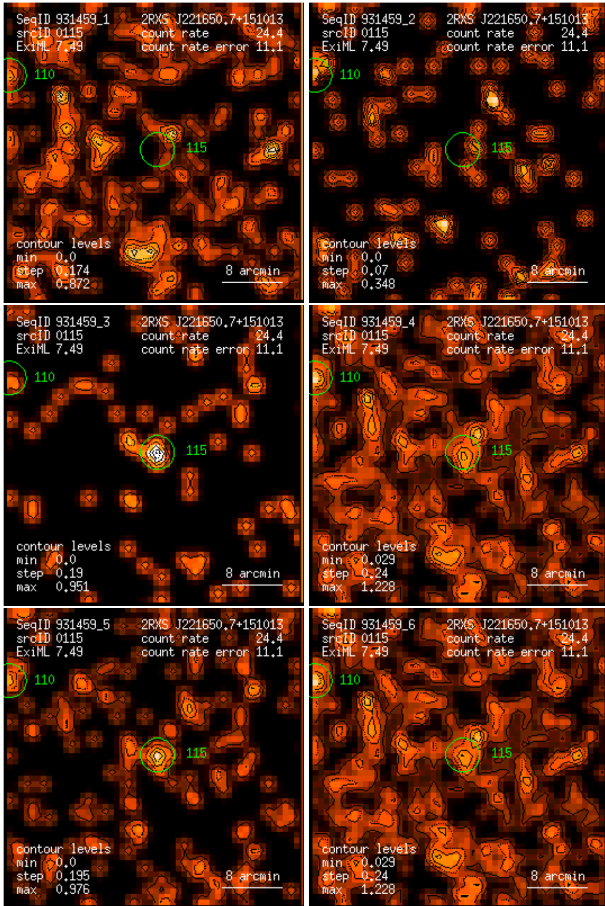
Figure 115: RASS 931459: detection 0115: band rate images, Gaussian filter: (1) PSPC channels 11 – 41, (2) 52 – 90, (3) 91 – 201, (4) 11 – 235, (5) 52 – 201, (6) 11 – 201. Broad band rates in counts/ks. Band rate contour levels in counts/ks/arcmin 2 .
