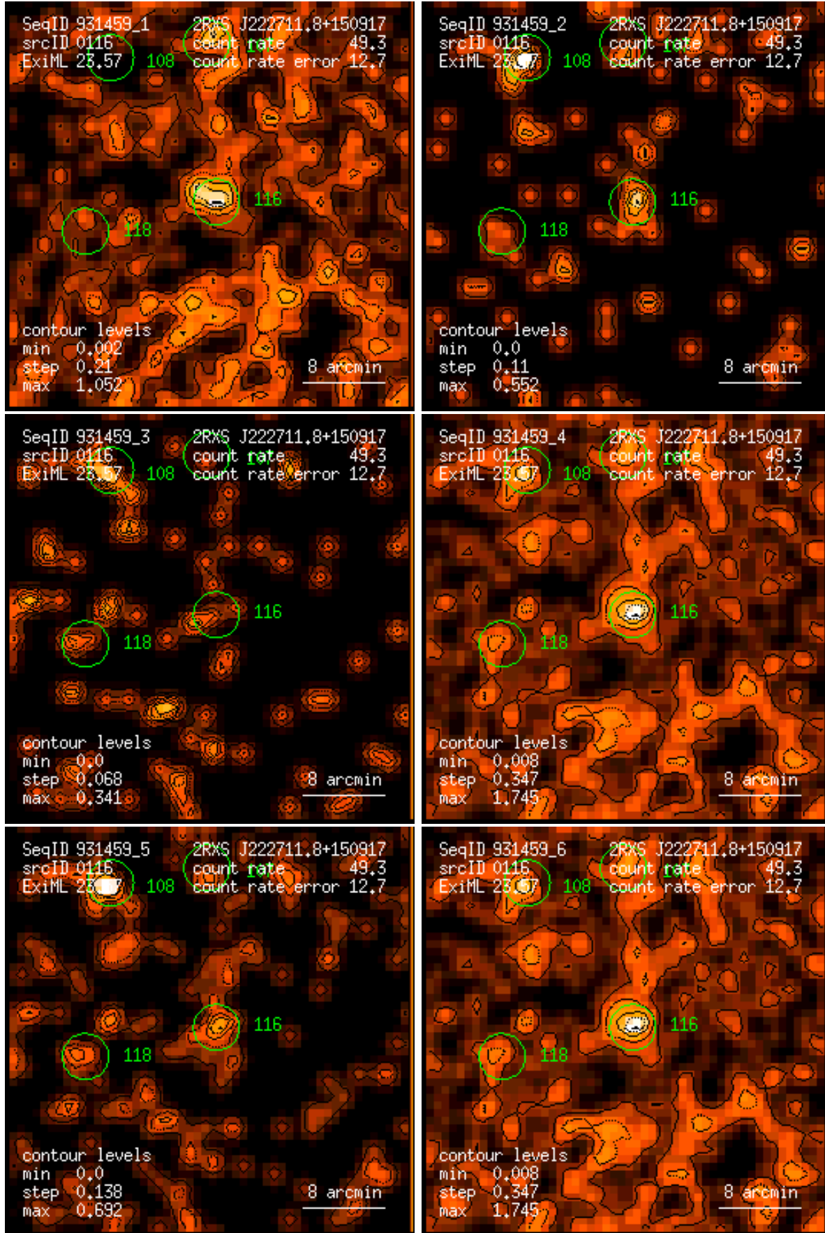
Figure 116: RASS 931459: detection 0116: band rate images, Gaussian filter: (1) PSPC channels 11 – 41, (2) 52 – 90, (3) 91 – 201, (4) 11 – 235, (5) 52 – 201, (6) 11 – 201. Broad band rates in counts/ks. Band rate contour levels in counts/ks/arcmin 2 .
