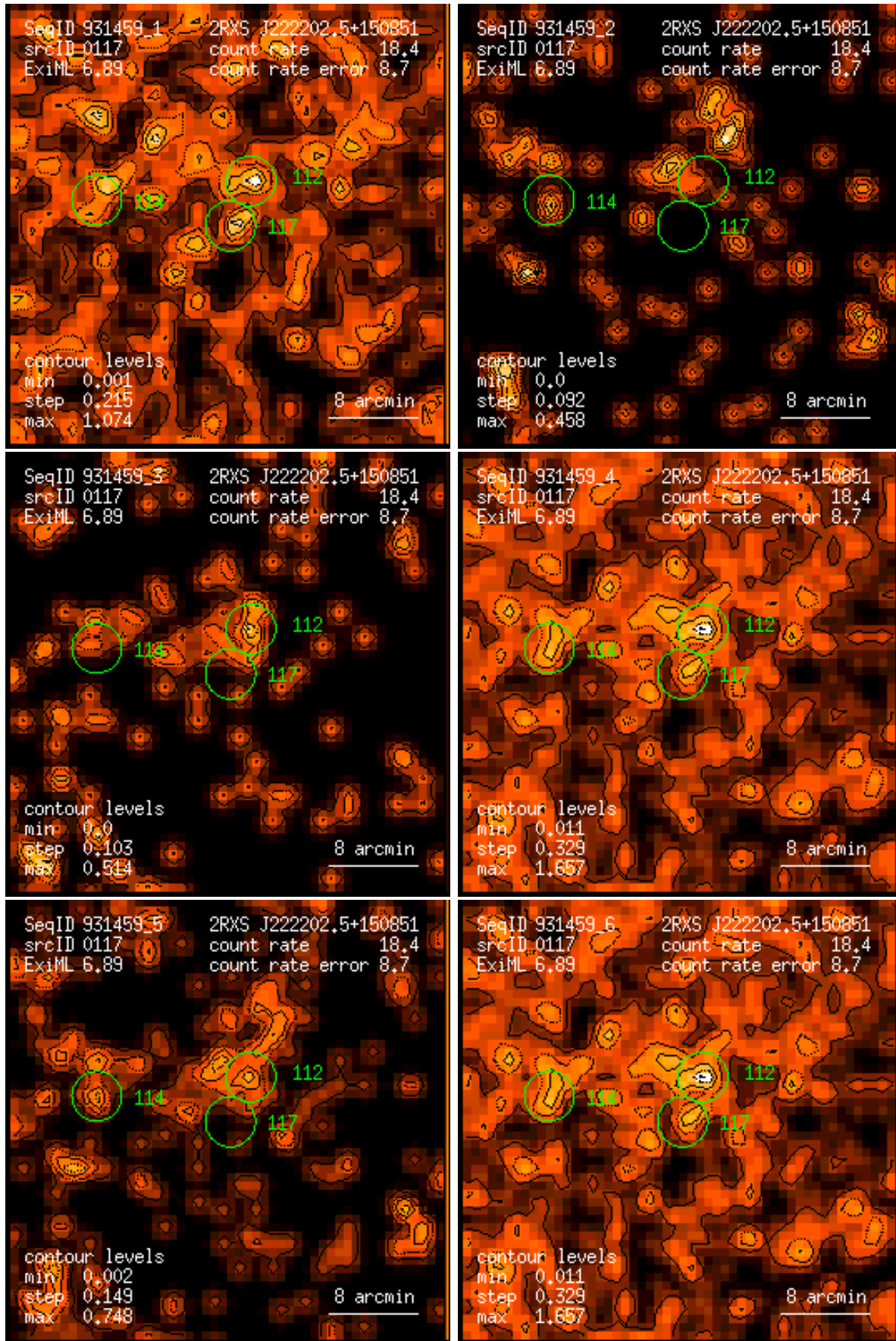
Figure 117: RASS 931459: detection 0117: band rate images, Gaussian filter: (1) PSPC channels 11 – 41, (2) 52 – 90, (3) 91 – 201, (4) 11 – 235, (5) 52 – 201, (6) 11 – 201. Broad band rates in counts/ks. Band rate contour levels in counts/ks/arcmin 2 .
