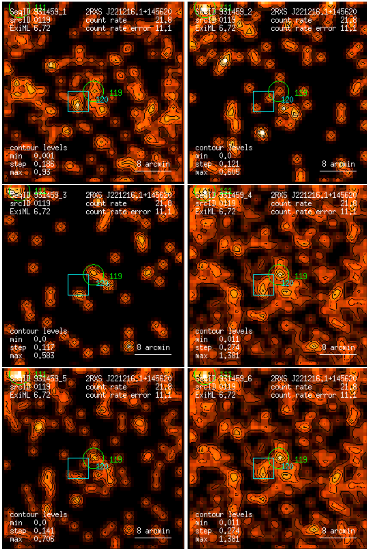
Figure 119: RASS 931459: detection 0119: band rate images, Gaussian filter: (1) PSPC channels 11 – 41, (2) 52 – 90, (3) 91 – 201, (4) 11 – 235, (5) 52 – 201, (6) 11 – 201. Broad band rates in counts/ks. Band rate contour levels in counts/ks/arcmin 2 .
