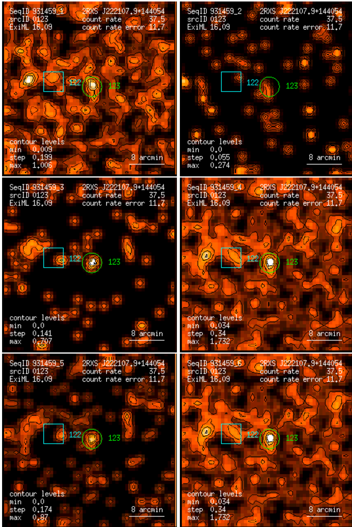
Figure 123: RASS 931459: detection 0123: band rate images, Gaussian filter: (1) PSPC channels 11 – 41, (2) 52 – 90, (3) 91 – 201, (4) 11 – 235, (5) 52 – 201, (6) 11 – 201. Broad band rates in counts/ks. Band rate contour levels in counts/ks/arcmin 2 .
