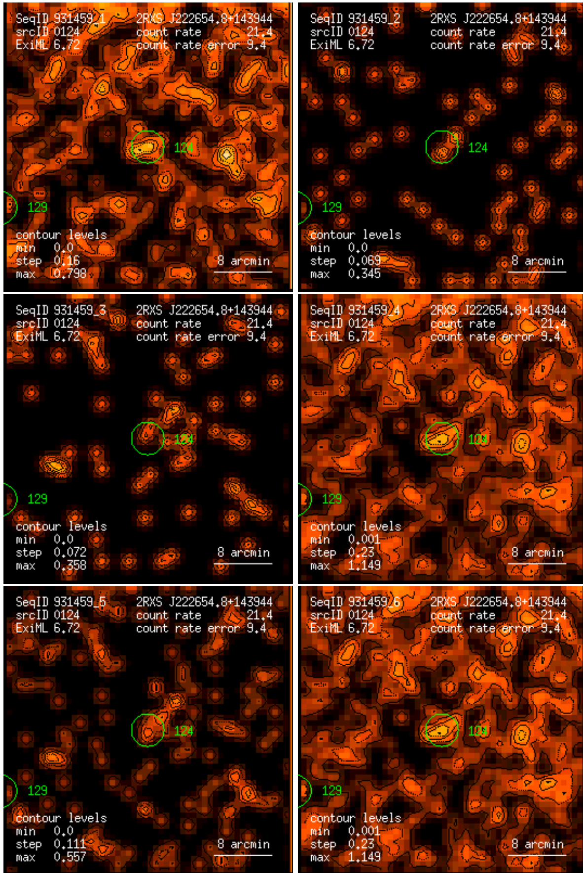
Figure 124: RASS 931459: detection 0124: band rate images, Gaussian filter: (1) PSPC channels 11 – 41, (2) 52 – 90, (3) 91 – 201, (4) 11 – 235, (5) 52 – 201, (6) 11 – 201. Broad band rates in counts/ks. Band rate contour levels in counts/ks/arcmin 2 .
