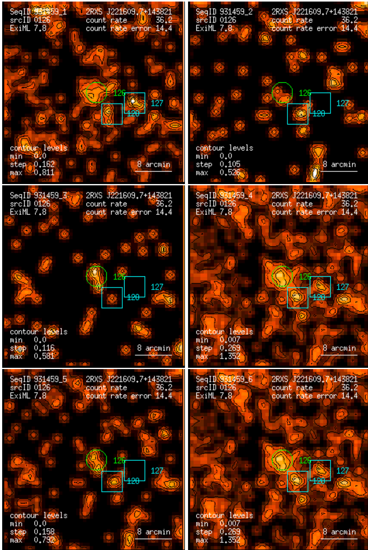
Figure 126: RASS 931459: detection 0126: band rate images, Gaussian filter: (1) PSPC channels 11 – 41, (2) 52 – 90, (3) 91 – 201, (4) 11 – 235, (5) 52 – 201, (6) 11 – 201. Broad band rates in counts/ks. Band rate contour levels in counts/ks/arcmin 2 .
