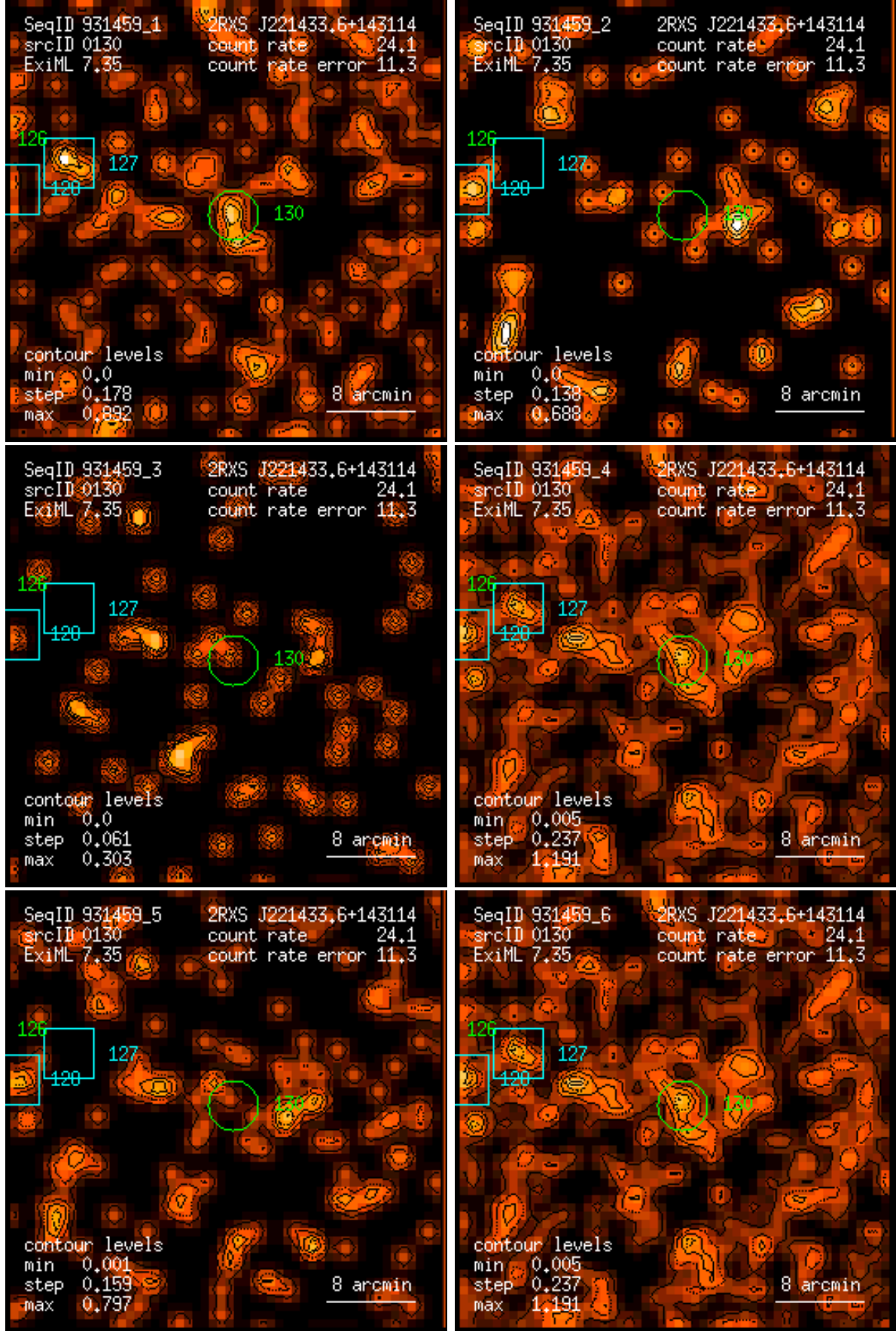
Figure 130: RASS 931459: detection 0130: band rate images, Gaussian filter: (1) PSPC channels 11 – 41, (2) 52 – 90, (3) 91 – 201, (4) 11 – 235, (5) 52 – 201, (6) 11 – 201. Broad band rates in counts/ks. Band rate contour levels in counts/ks/arcmin 2 .
