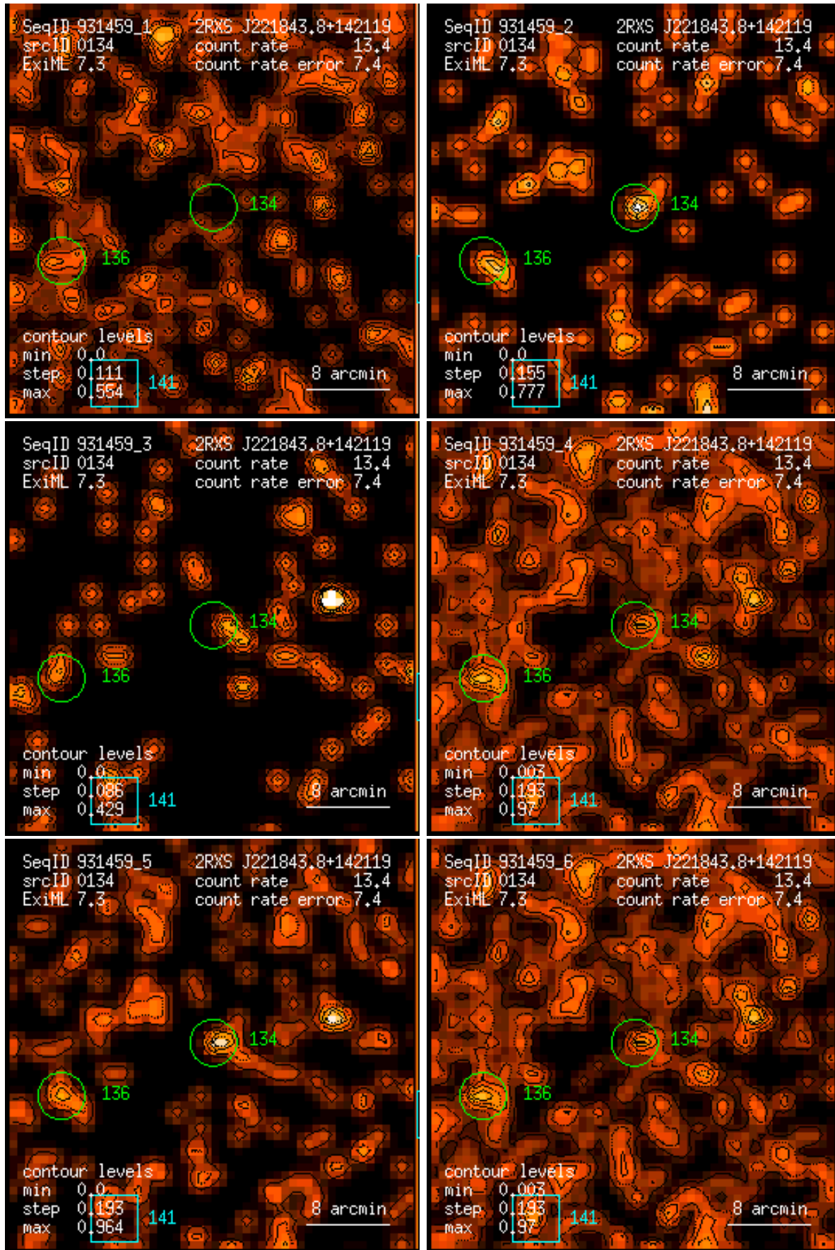
Figure 134: RASS 931459: detection 0134: band rate images, Gaussian filter: (1) PSPC channels 11 – 41, (2) 52 – 90, (3) 91 – 201, (4) 11 – 235, (5) 52 – 201, (6) 11 – 201. Broad band rates in counts/ks. Band rate contour levels in counts/ks/arcmin 2 .
