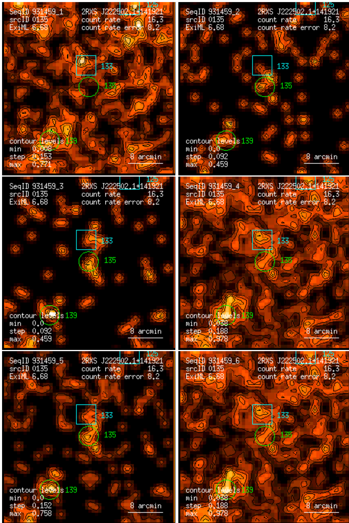
Figure 135: RASS 931459: detection 0135: band rate images, Gaussian filter: (1) PSPC channels 11 – 41, (2) 52 – 90, (3) 91 – 201, (4) 11 – 235, (5) 52 – 201, (6) 11 – 201. Broad band rates in counts/ks. Band rate contour levels in counts/ks/arcmin 2 .
