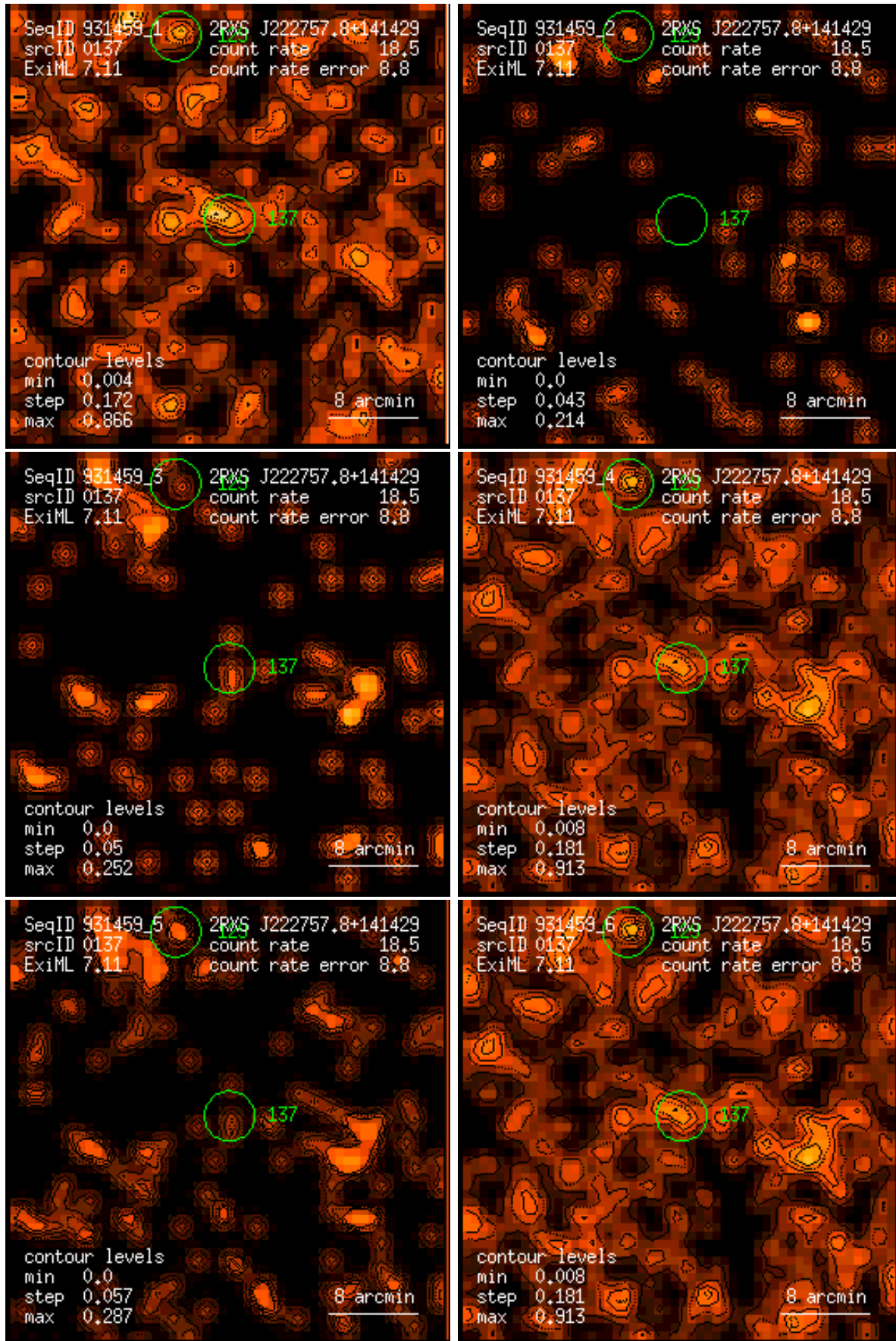
Figure 137: RASS 931459: detection 0137: band rate images, Gaussian filter: (1) PSPC channels 11 – 41, (2) 52 – 90, (3) 91 – 201, (4) 11 – 235, (5) 52 – 201, (6) 11 – 201. Broad band rates in counts/ks. Band rate contour levels in counts/ks/arcmin 2 .
