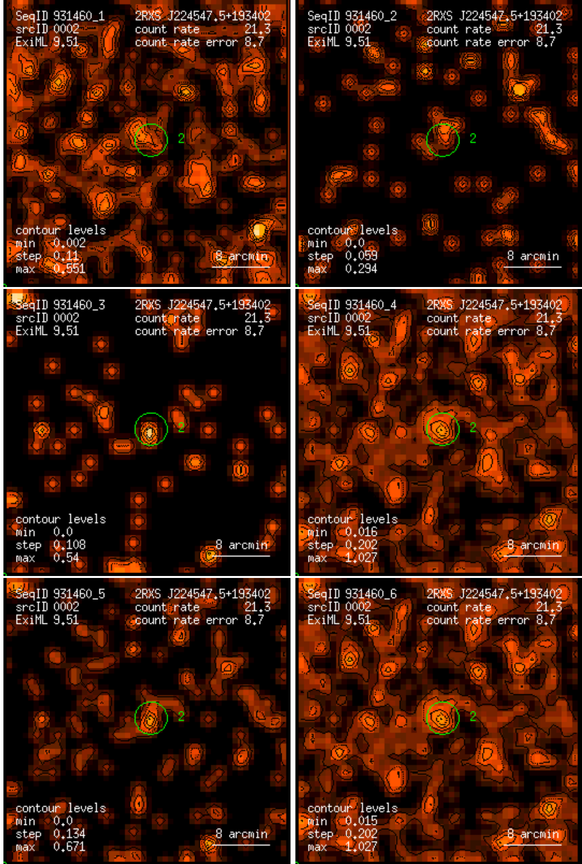
Figure 2: RASS 931460: detection 0002: band rate images, Gaussian filter: (1) PSPC channels 11 – 41, (2) 52 – 90, (3) 91 – 201, (4) 11 – 235, (5) 52 – 201, (6) 11 – 201. Broad band rates in counts/ks. Band rate contour levels in counts/ks/arcmin 2 .
