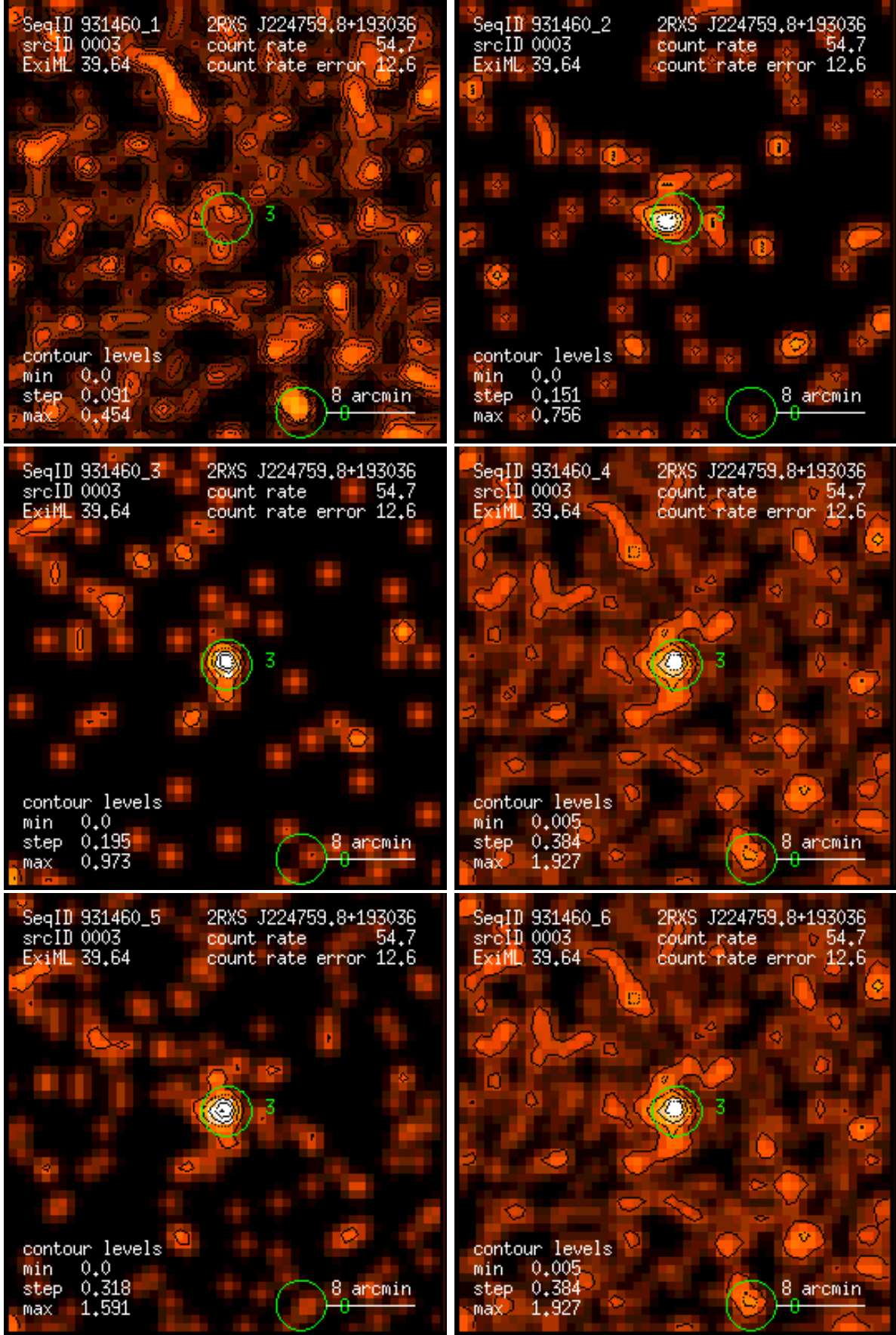
Figure 3: RASS 931460: detection 0003: band rate images, Gaussian filter: (1) PSPC channels 11 – 41, (2) 52 – 90, (3) 91 – 201, (4) 11 – 235, (5) 52 – 201, (6) 11 – 201. Broad band rates in counts/ks. Band rate contour levels in counts/ks/arcmin 2 .
