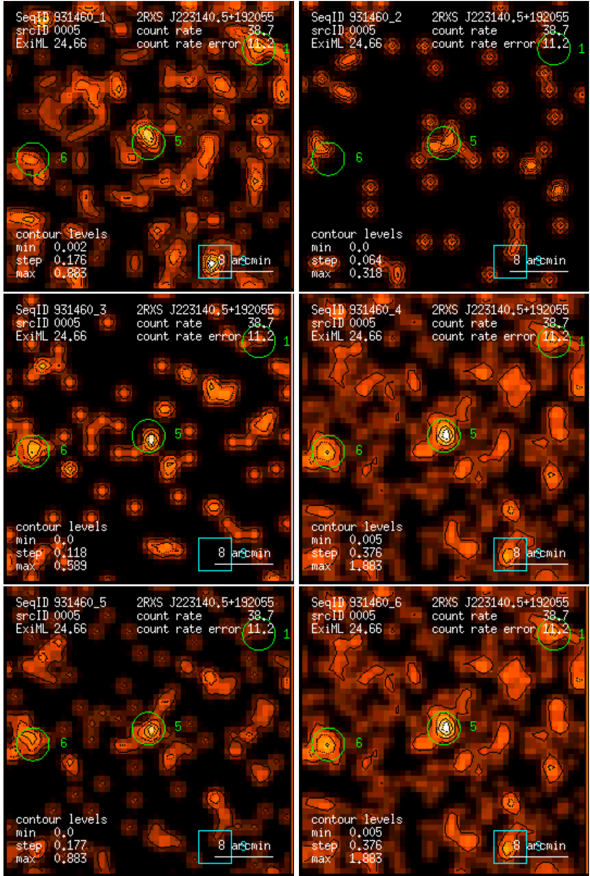
Figure 5: RASS 931460: detection 0005: band rate images, Gaussian filter: (1) PSPC channels 11 – 41, (2) 52 – 90, (3) 91 – 201, (4) 11 – 235, (5) 52 – 201, (6) 11 – 201. Broad band rates in counts/ks. Band rate contour levels in counts/ks/arcmin 2 .
