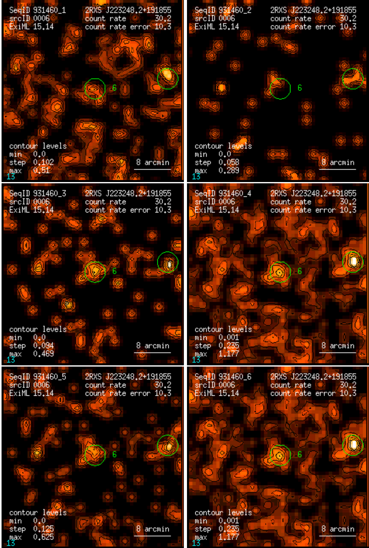
Figure 6: RASS 931460: detection 0006: band rate images, Gaussian filter: (1) PSPC channels 11 – 41, (2) 52 – 90, (3) 91 – 201, (4) 11 – 235, (5) 52 – 201, (6) 11 – 201. Broad band rates in counts/ks. Band rate contour levels in counts/ks/arcmin 2 .
