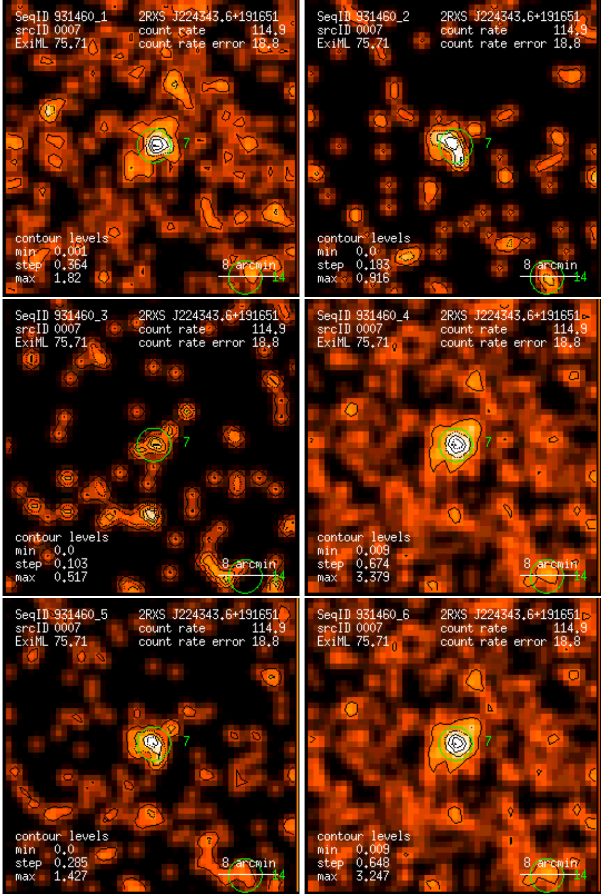
Figure 7: RASS 931460: detection 0007: band rate images, Gaussian filter: (1) PSPC channels 11 – 41, (2) 52 – 90, (3) 91 – 201, (4) 11 – 235, (5) 52 – 201, (6) 11 – 201. Broad band rates in counts/ks. Band rate contour levels in counts/ks/arcmin 2 .
