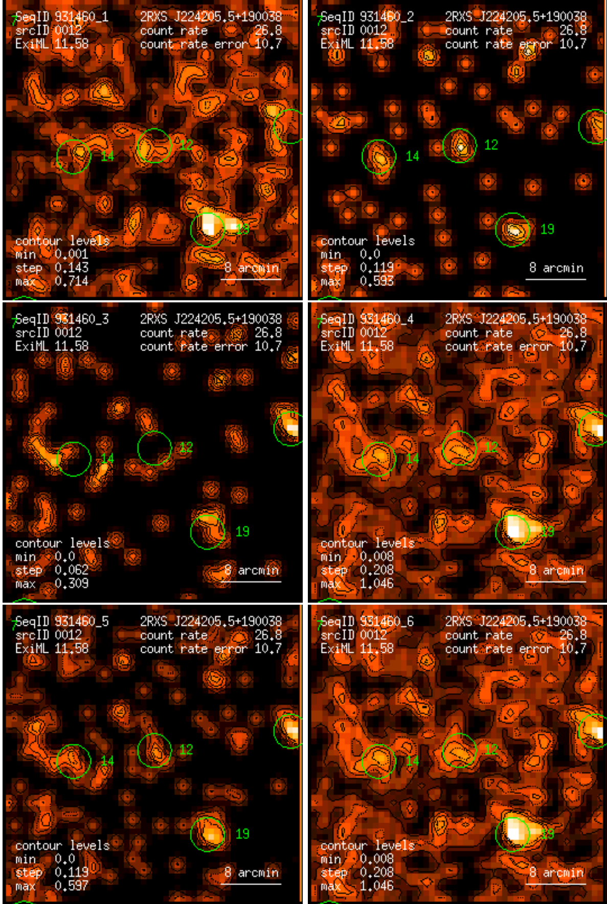
Figure 12: RASS 931460: detection 0012: band rate images, Gaussian filter: (1) PSPC channels 11 – 41, (2) 52 – 90, (3) 91 – 201, (4) 11 – 235, (5) 52 – 201, (6) 11 – 201. Broad band rates in counts/ks. Band rate contour levels in counts/ks/arcmin 2 .
