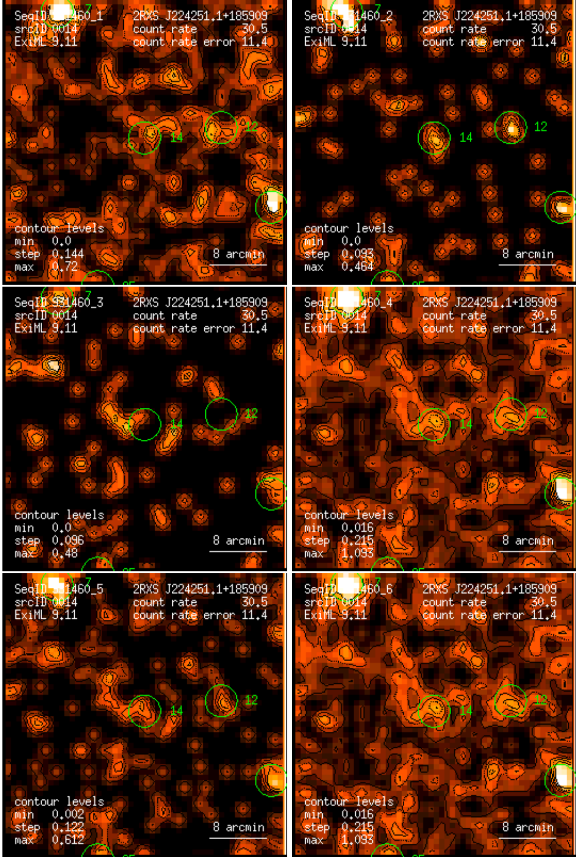
Figure 14: RASS 931460: detection 0014: band rate images, Gaussian filter: (1) PSPC channels 11 – 41, (2) 52 – 90, (3) 91 – 201, (4) 11 – 235, (5) 52 – 201, (6) 11 – 201. Broad band rates in counts/ks. Band rate contour levels in counts/ks/arcmin 2 .
