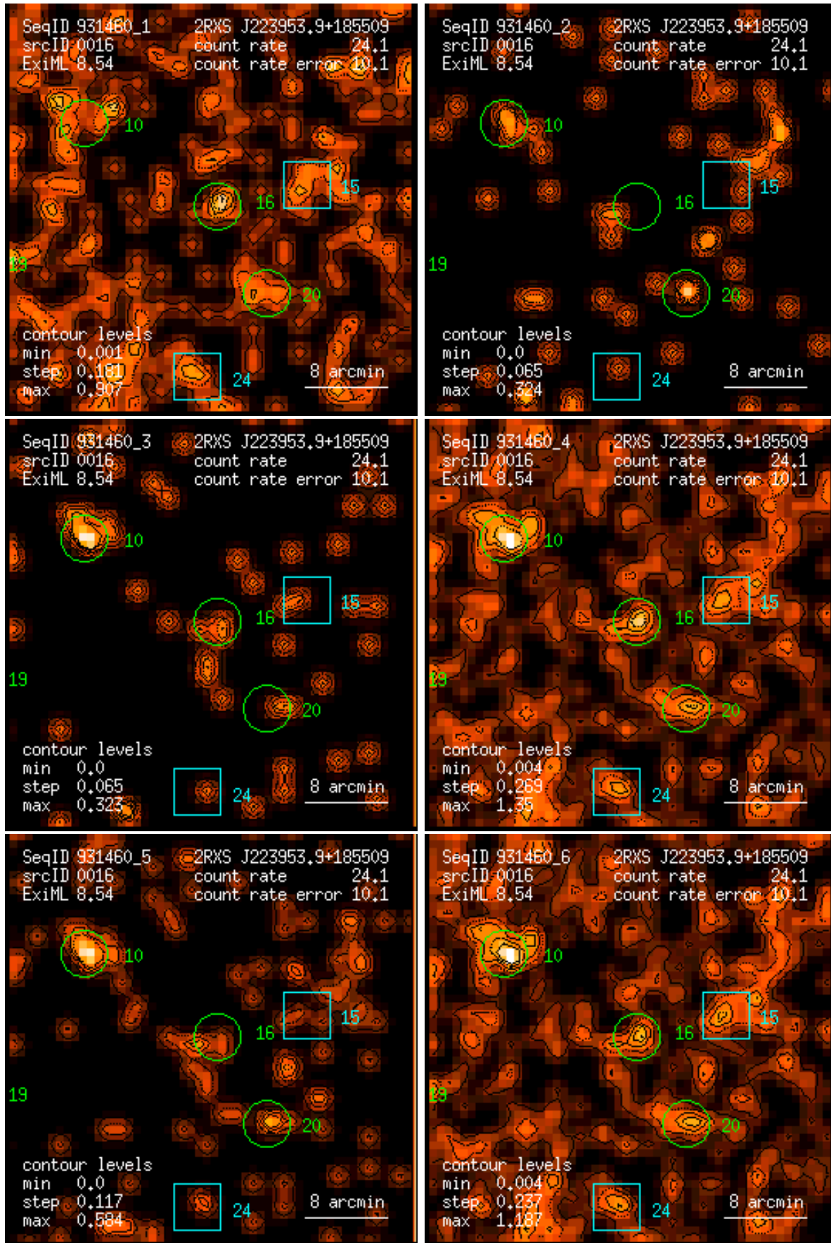
Figure 16: RASS 931460: detection 0016: band rate images, Gaussian filter: (1) PSPC channels 11 – 41, (2) 52 – 90, (3) 91 – 201, (4) 11 – 235, (5) 52 – 201, (6) 11 – 201. Broad band rates in counts/ks. Band rate contour levels in counts/ks/arcmin 2 .
