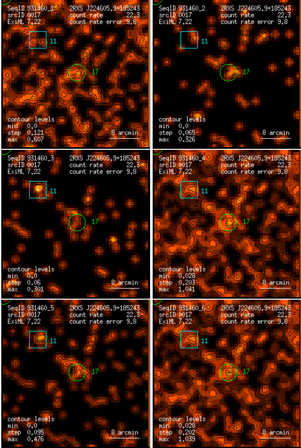
Figure 17: RASS 931460: detection 0017: band rate images, Gaussian filter: (1) PSPC channels 11 – 41, (2) 52 – 90, (3) 91 – 201, (4) 11 – 235, (5) 52 – 201, (6) 11 – 201. Broad band rates in counts/ks. Band rate contour levels in counts/ks/arcmin 2 .
