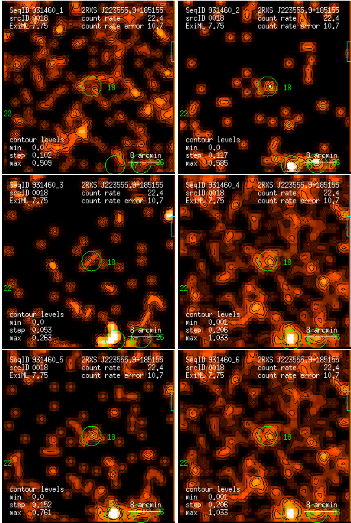
Figure 18: RASS 931460: detection 0018: band rate images, Gaussian filter: (1) PSPC channels 11 – 41, (2) 52 – 90, (3) 91 – 201, (4) 11 – 235, (5) 52 – 201, (6) 11 – 201. Broad band rates in counts/ks. Band rate contour levels in counts/ks/arcmin 2 .
