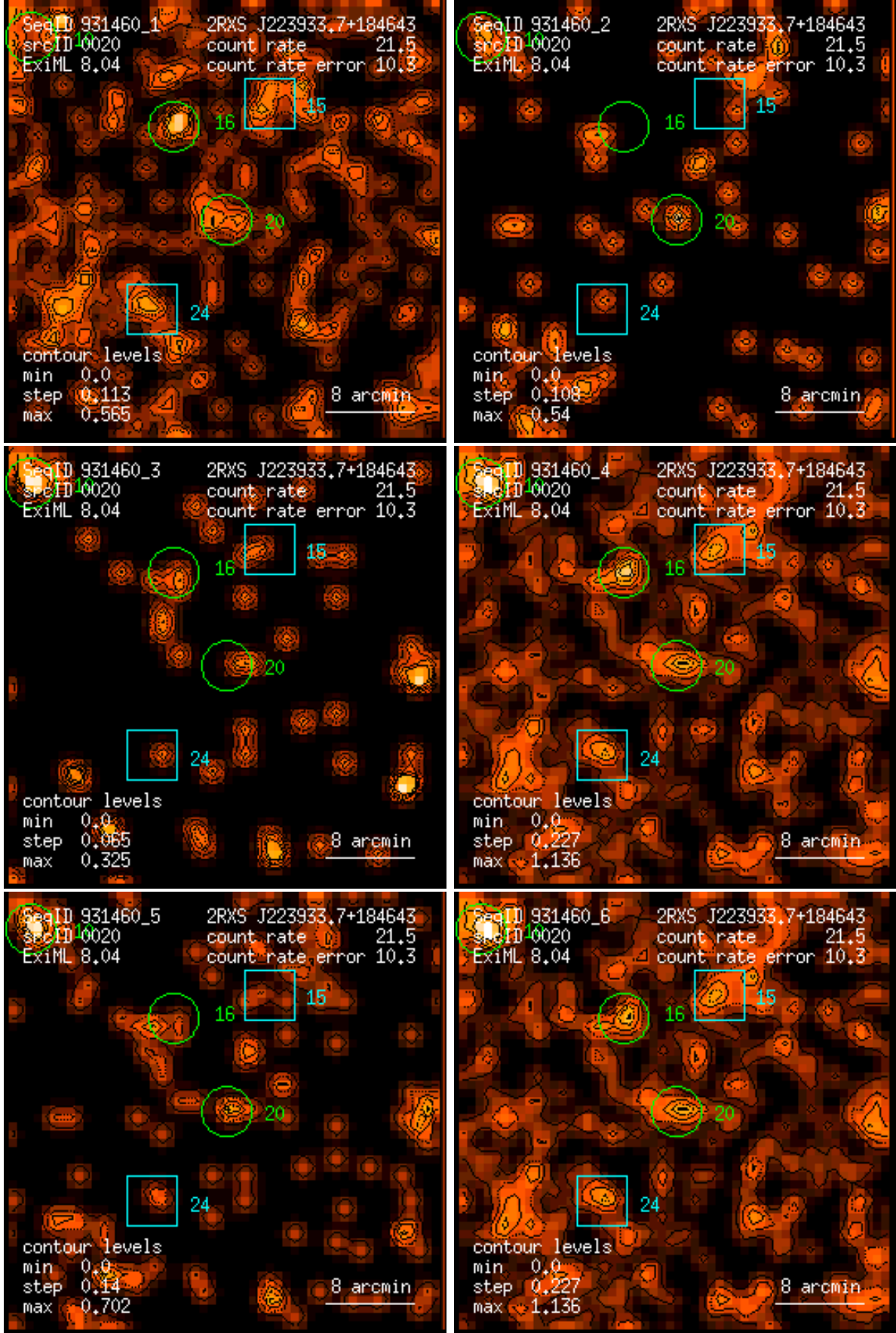
Figure 20: RASS 931460: detection 0020: band rate images, Gaussian filter: (1) PSPC channels 11 – 41, (2) 52 – 90, (3) 91 – 201, (4) 11 – 235, (5) 52 – 201, (6) 11 – 201. Broad band rates in counts/ks. Band rate contour levels in counts/ks/arcmin 2 .
