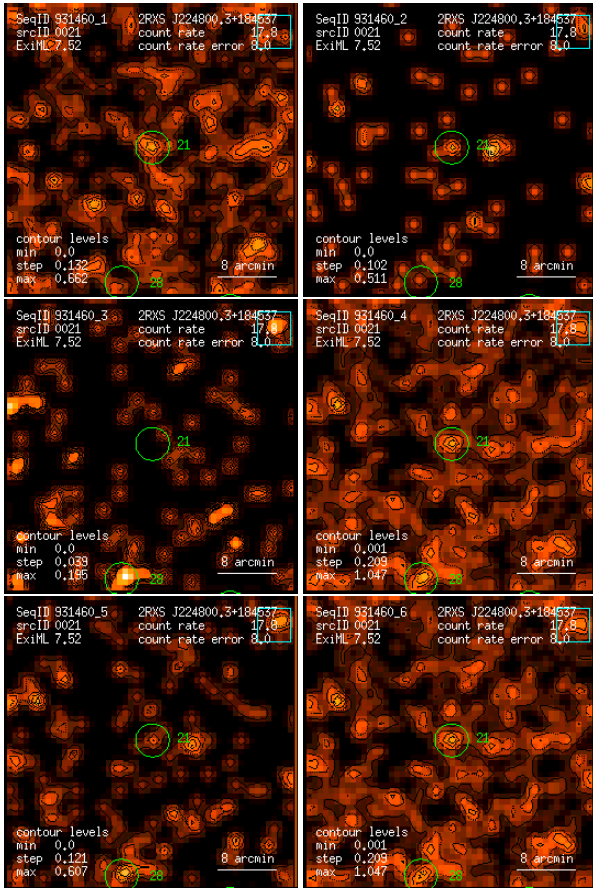
Figure 21: RASS 931460: detection 0021: band rate images, Gaussian filter: (1) PSPC channels 11 – 41, (2) 52 – 90, (3) 91 – 201, (4) 11 – 235, (5) 52 – 201, (6) 11 – 201. Broad band rates in counts/ks. Band rate contour levels in counts/ks/arcmin 2 .
