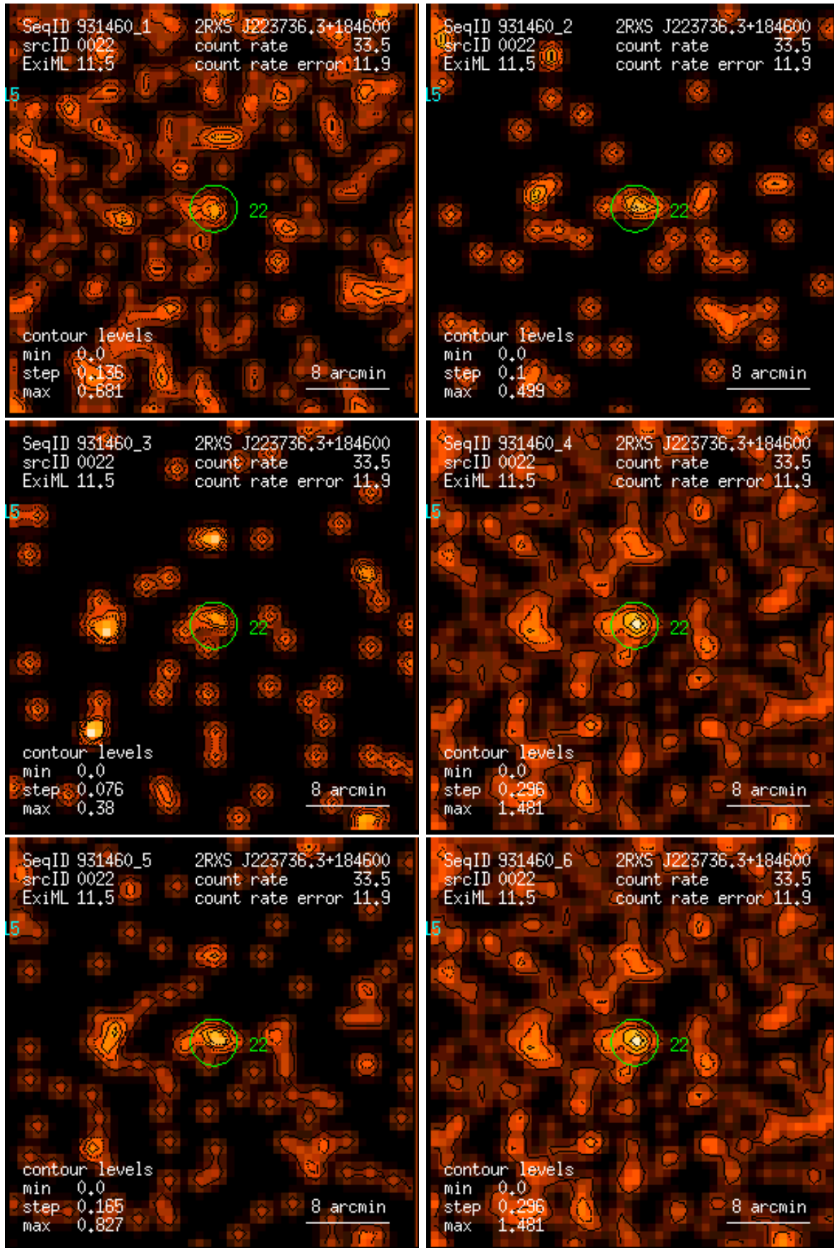
Figure 22: RASS 931460: detection 0022: band rate images, Gaussian filter: (1) PSPC channels 11 – 41, (2) 52 – 90, (3) 91 – 201, (4) 11 – 235, (5) 52 – 201, (6) 11 – 201. Broad band rates in counts/ks. Band rate contour levels in counts/ks/arcmin 2 .
