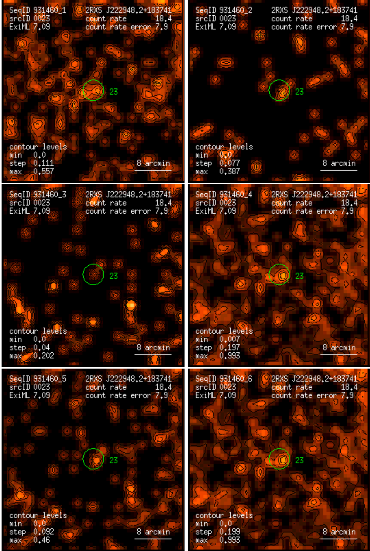
Figure 23: RASS 931460: detection 0023: band rate images, Gaussian filter: (1) PSPC channels 11 – 41, (2) 52 – 90, (3) 91 – 201, (4) 11 – 235, (5) 52 – 201, (6) 11 – 201. Broad band rates in counts/ks. Band rate contour levels in counts/ks/arcmin 2 .
