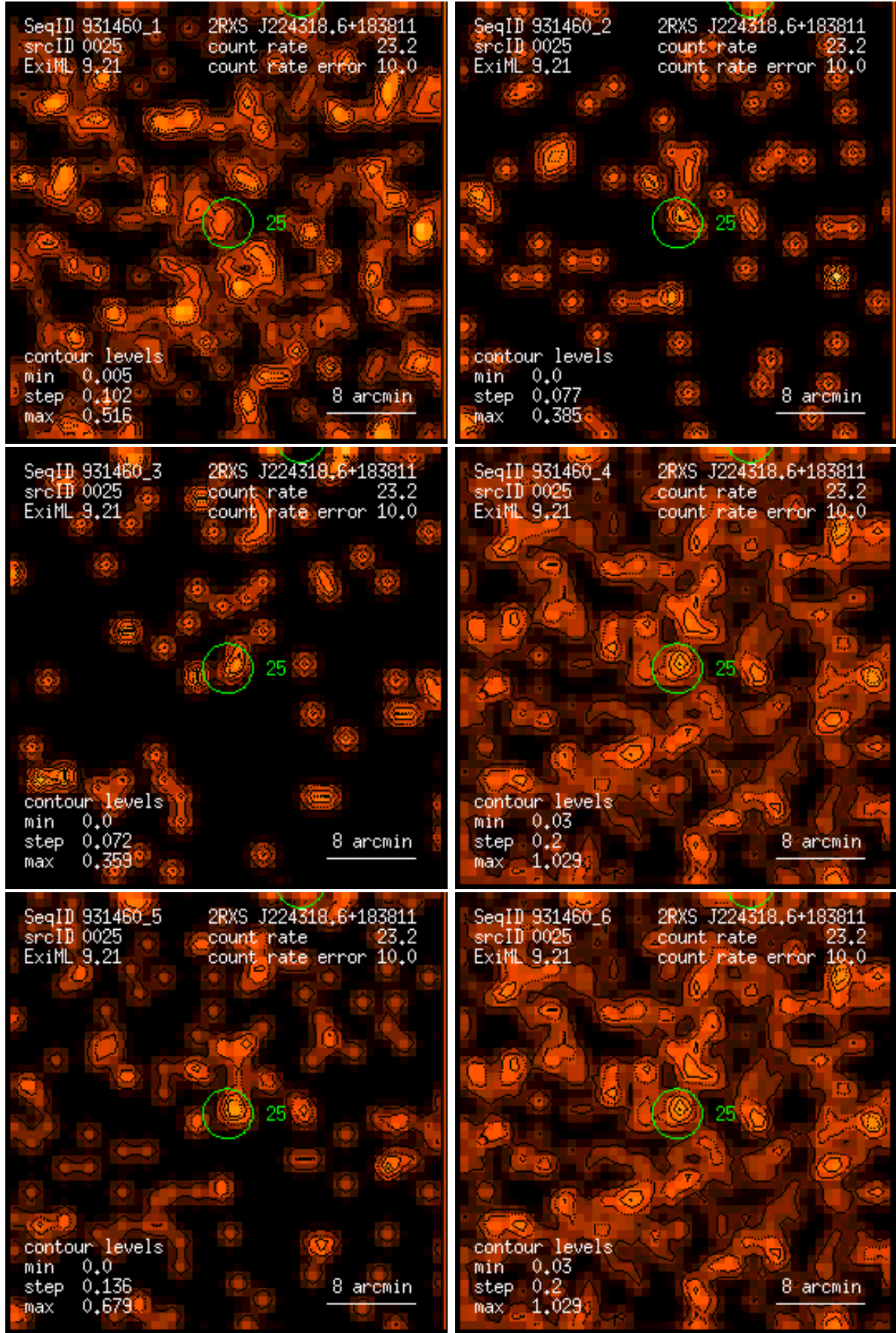
Figure 25: RASS 931460: detection 0025: band rate images, Gaussian filter: (1) PSPC channels 11 – 41, (2) 52 – 90, (3) 91 – 201, (4) 11 – 235, (5) 52 – 201, (6) 11 – 201. Broad band rates in counts/ks. Band rate contour levels in counts/ks/arcmin 2 .
