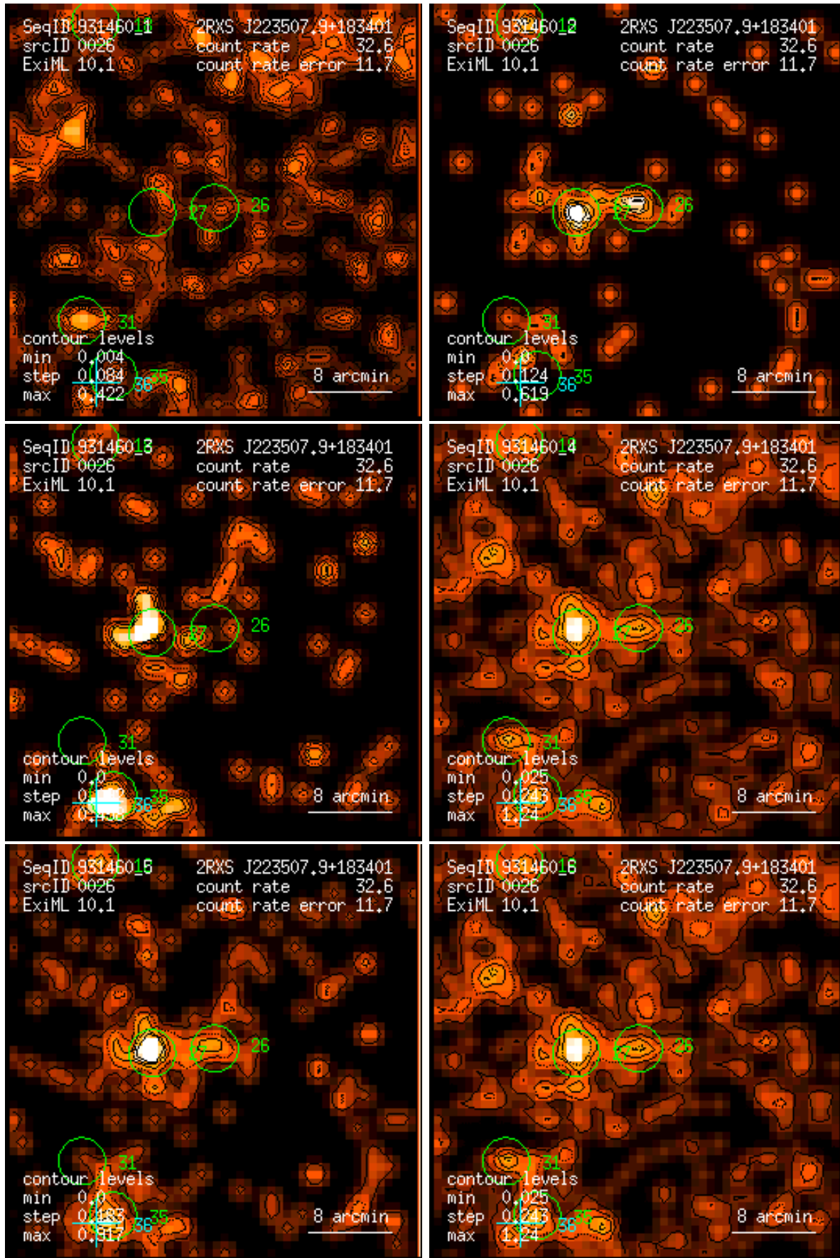
Figure 26: RASS 931460: detection 0026: band rate images, Gaussian filter: (1) PSPC channels 11 – 41, (2) 52 – 90, (3) 91 – 201, (4) 11 – 235, (5) 52 – 201, (6) 11 – 201. Broad band rates in counts/ks. Band rate contour levels in counts/ks/arcmin 2 .
