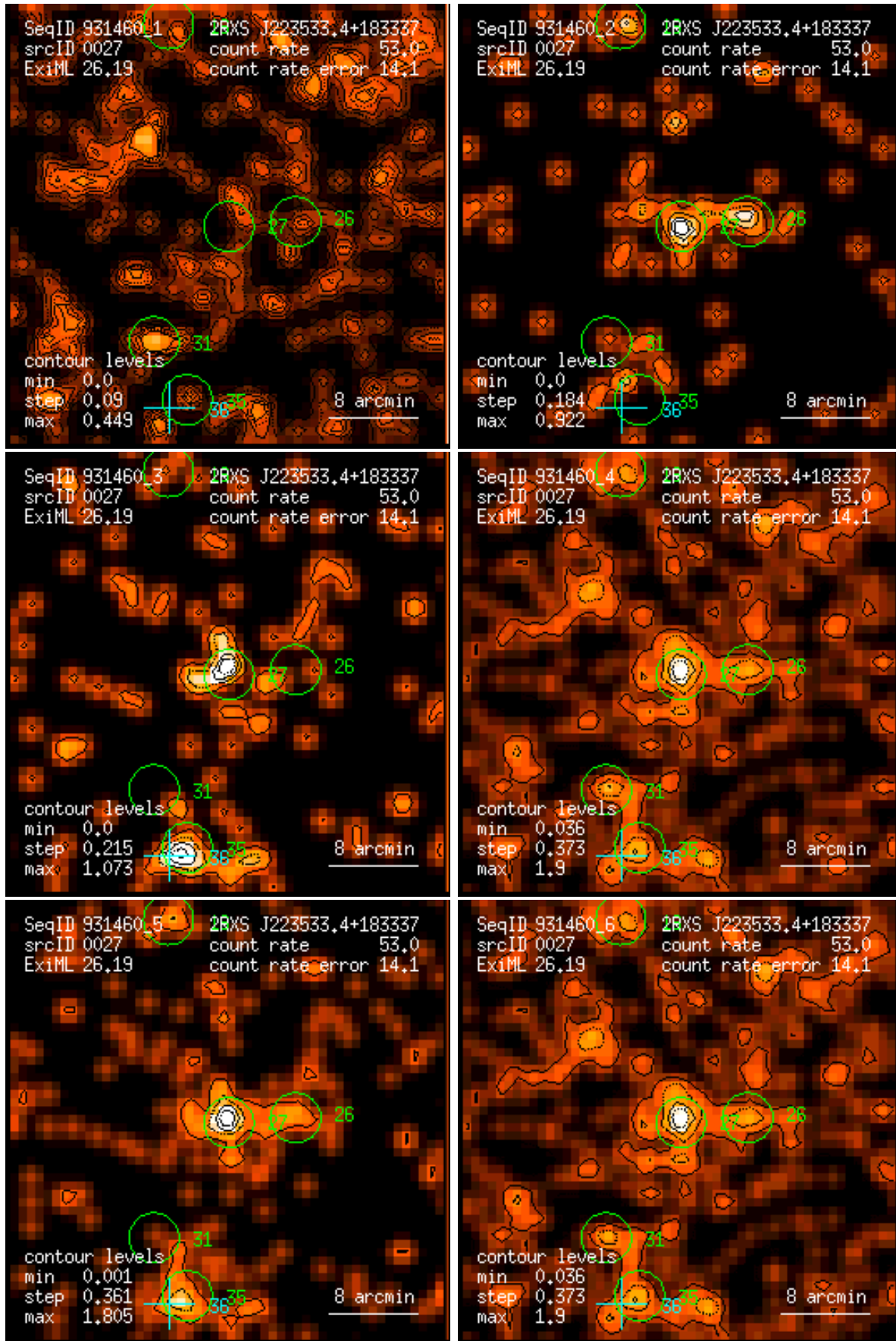
Figure 27: RASS 931460: detection 0027: band rate images, Gaussian filter: (1) PSPC channels 11 – 41, (2) 52 – 90, (3) 91 – 201, (4) 11 – 235, (5) 52 – 201, (6) 11 – 201. Broad band rates in counts/ks. Band rate contour levels in counts/ks/arcmin 2 .
