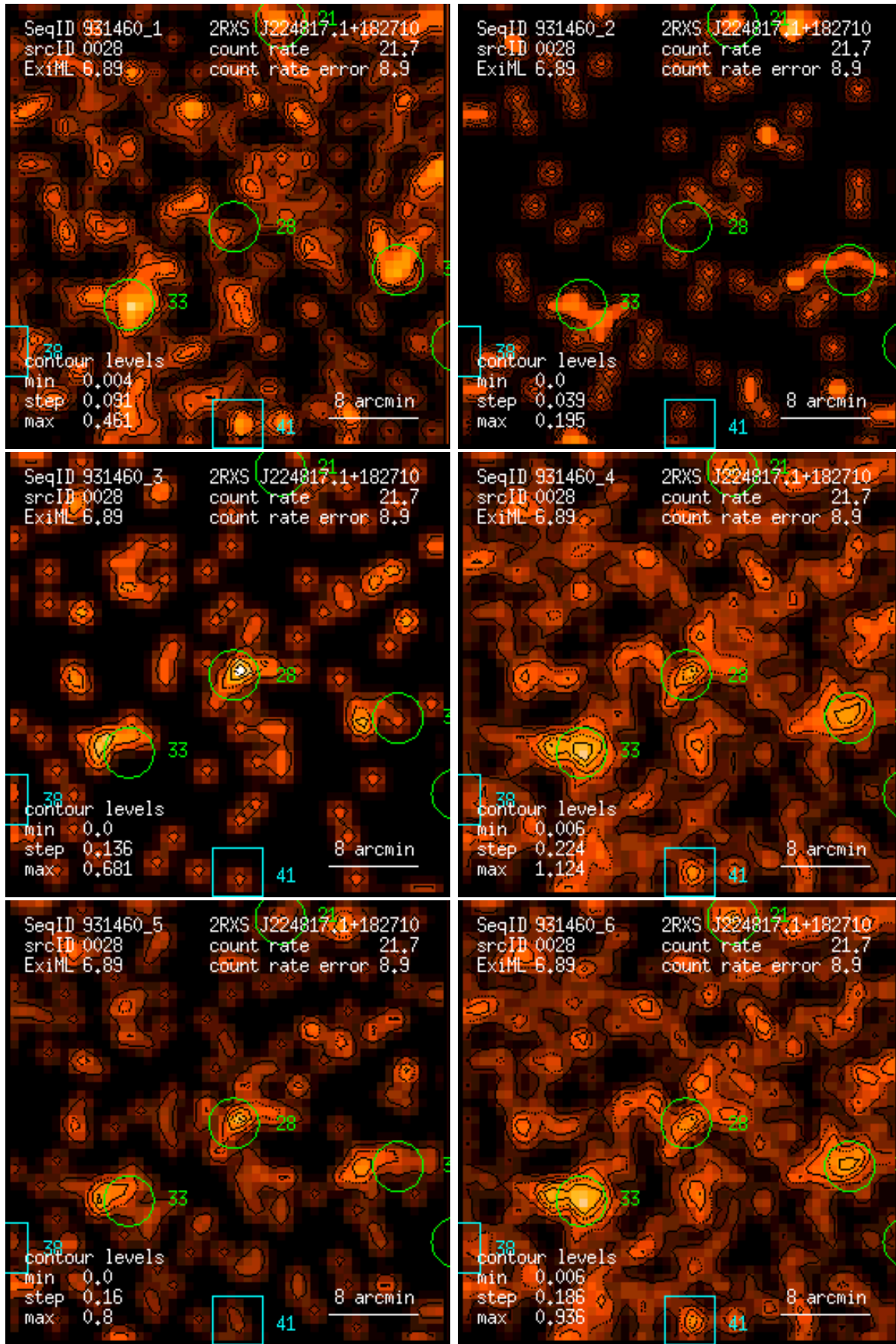
Figure 28: RASS 931460: detection 0028: band rate images, Gaussian filter: (1) PSPC channels 11 – 41, (2) 52 – 90, (3) 91 – 201, (4) 11 – 235, (5) 52 – 201, (6) 11 – 201. Broad band rates in counts/ks. Band rate contour levels in counts/ks/arcmin 2 .
