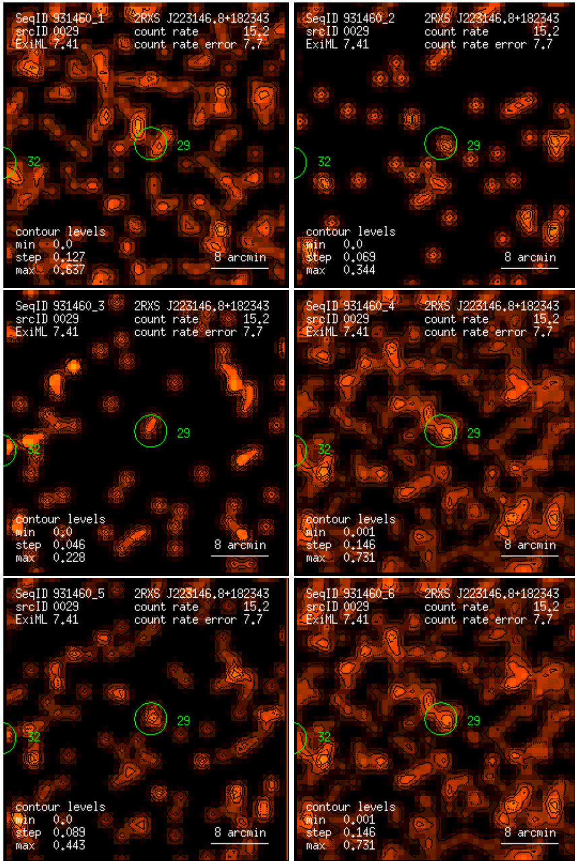
Figure 29: RASS 931460: detection 0029: band rate images, Gaussian filter: (1) PSPC channels 11 – 41, (2) 52 – 90, (3) 91 – 201, (4) 11 – 235, (5) 52 – 201, (6) 11 – 201. Broad band rates in counts/ks. Band rate contour levels in counts/ks/arcmin 2 .
