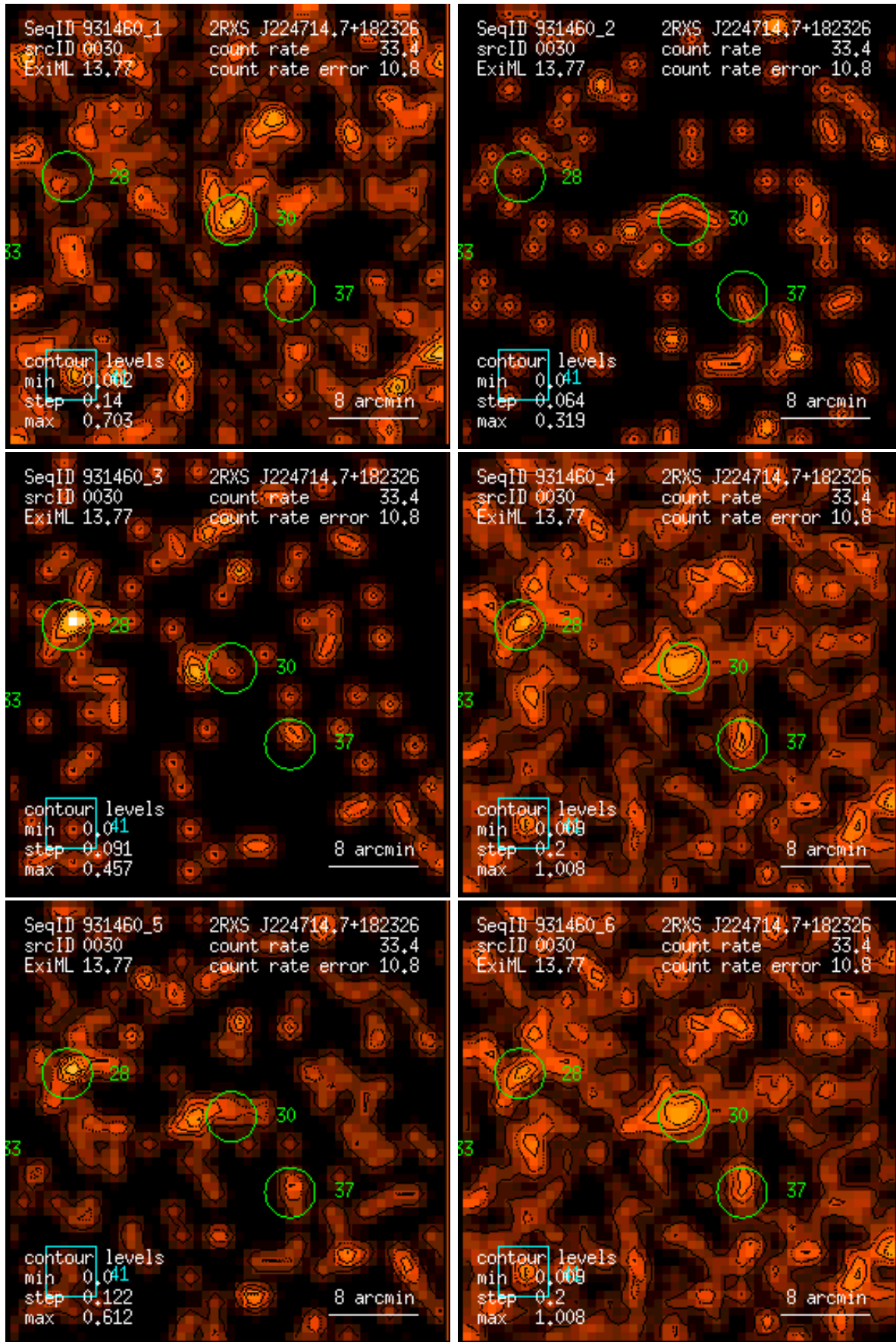
Figure 30: RASS 931460: detection 0030: band rate images, Gaussian filter: (1) PSPC channels 11 – 41, (2) 52 – 90, (3) 91 – 201, (4) 11 – 235, (5) 52 – 201, (6) 11 – 201. Broad band rates in counts/ks. Band rate contour levels in counts/ks/arcmin 2 .
