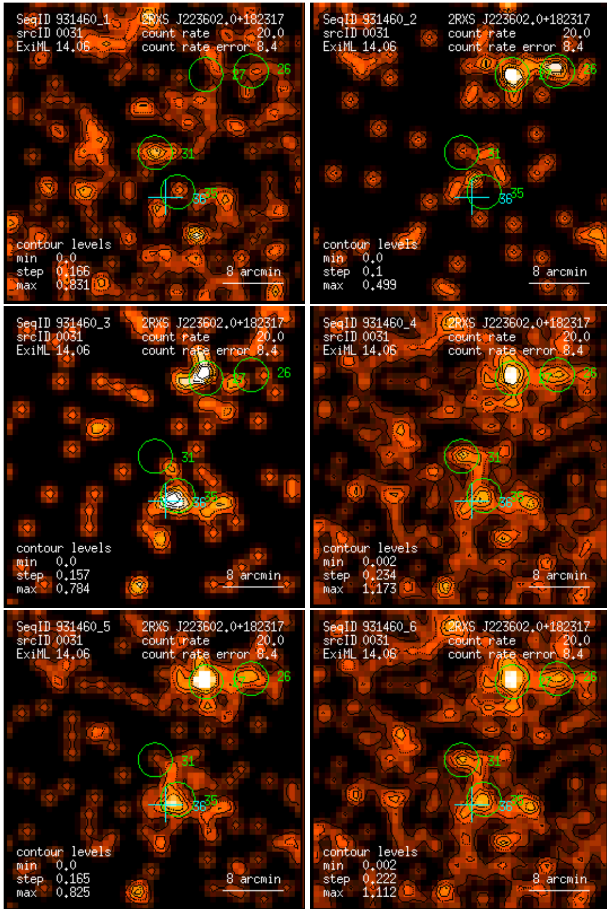
Figure 31: RASS 931460: detection 0031: band rate images, Gaussian filter: (1) PSPC channels 11 – 41, (2) 52 – 90, (3) 91 – 201, (4) 11 – 235, (5) 52 – 201, (6) 11 – 201. Broad band rates in counts/ks. Band rate contour levels in counts/ks/arcmin 2 .
